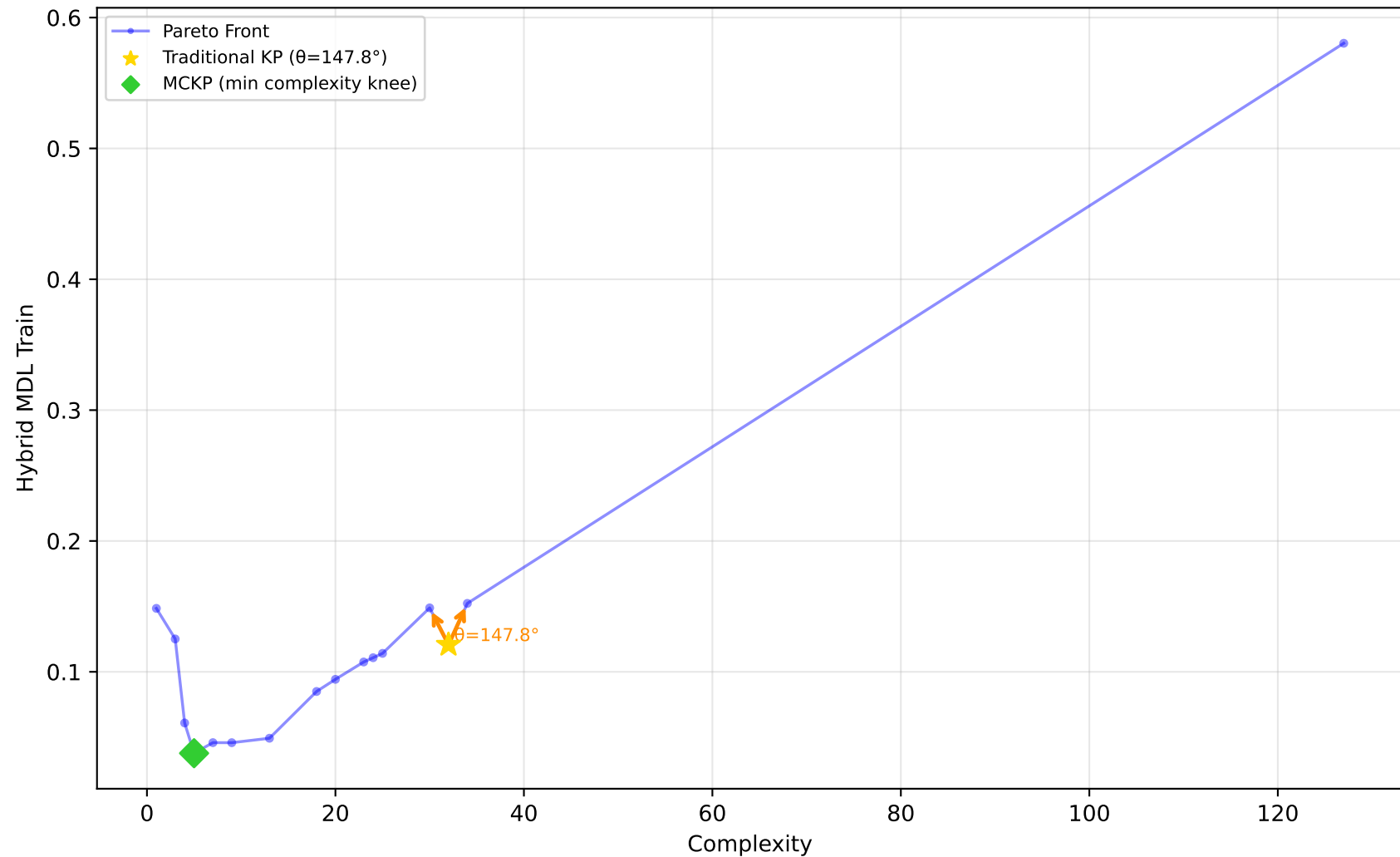
523_analcatdata_neavote - Run 24 - MVP - Hybrid MDL Train \lambda_1=0.00, \lambda_2=0.40, \lambda_3=0.00 | Difficulty: 1.00 | Method: hmr
