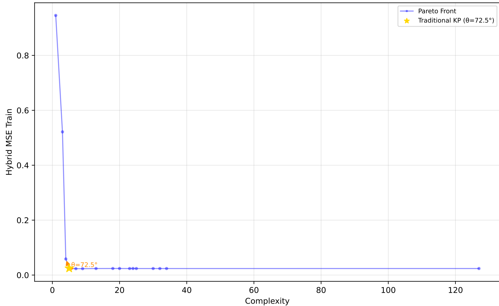
523_analcatdata_neavote - Run 24 - MVP - Hybrid MSE Train \lambda_1=0.00, \lambda_2=0.10, \lambda_3=0.00 | Difficulty: 1.00 | Method: hmr
