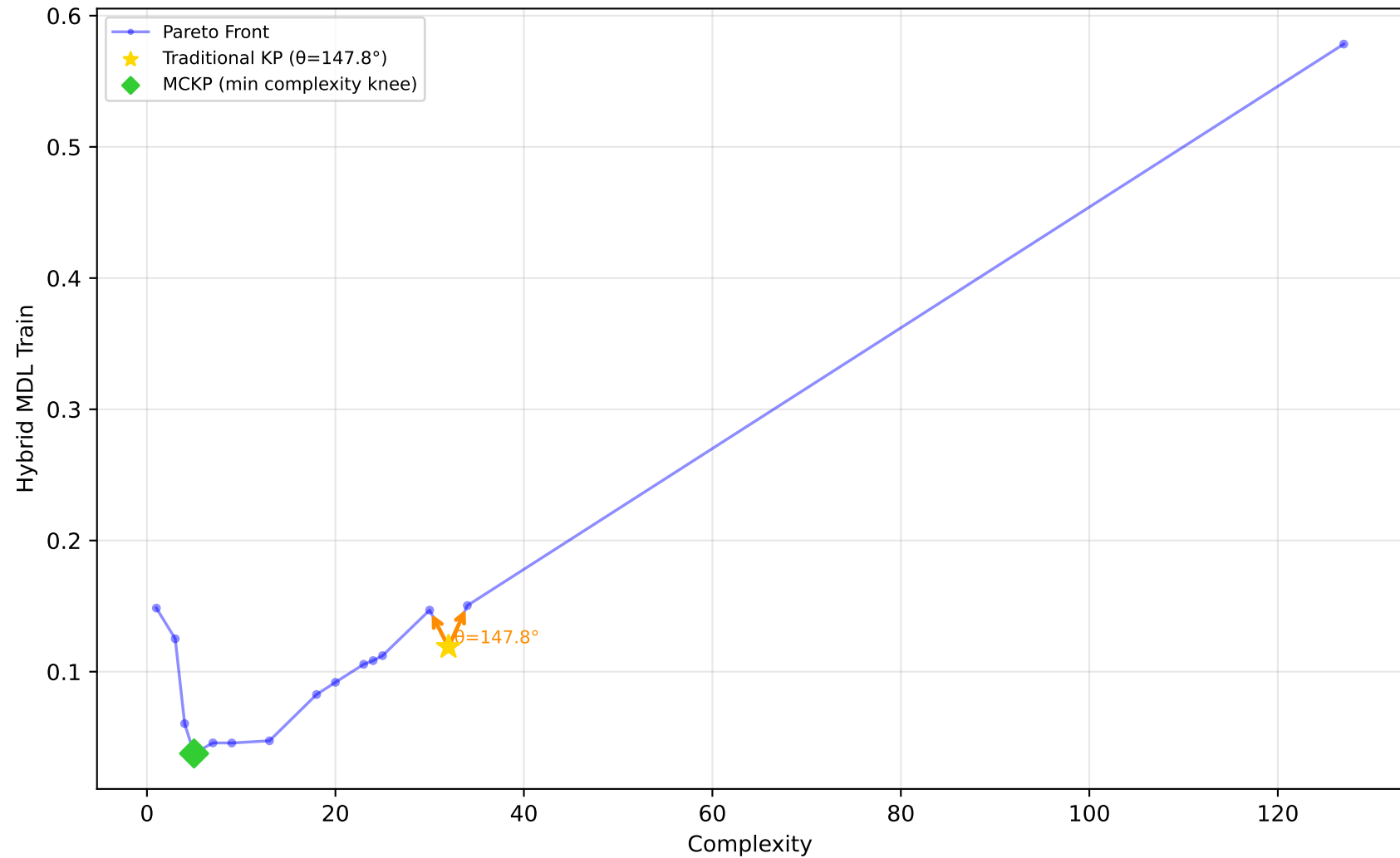
523_analcatdata_neavote - Run 24 - SVP - Hybrid MDL Train \lambda_1=0.00, \lambda_2=0.20, \lambda_3=0.00 | Difficulty: 1.00 | Method: hmr
