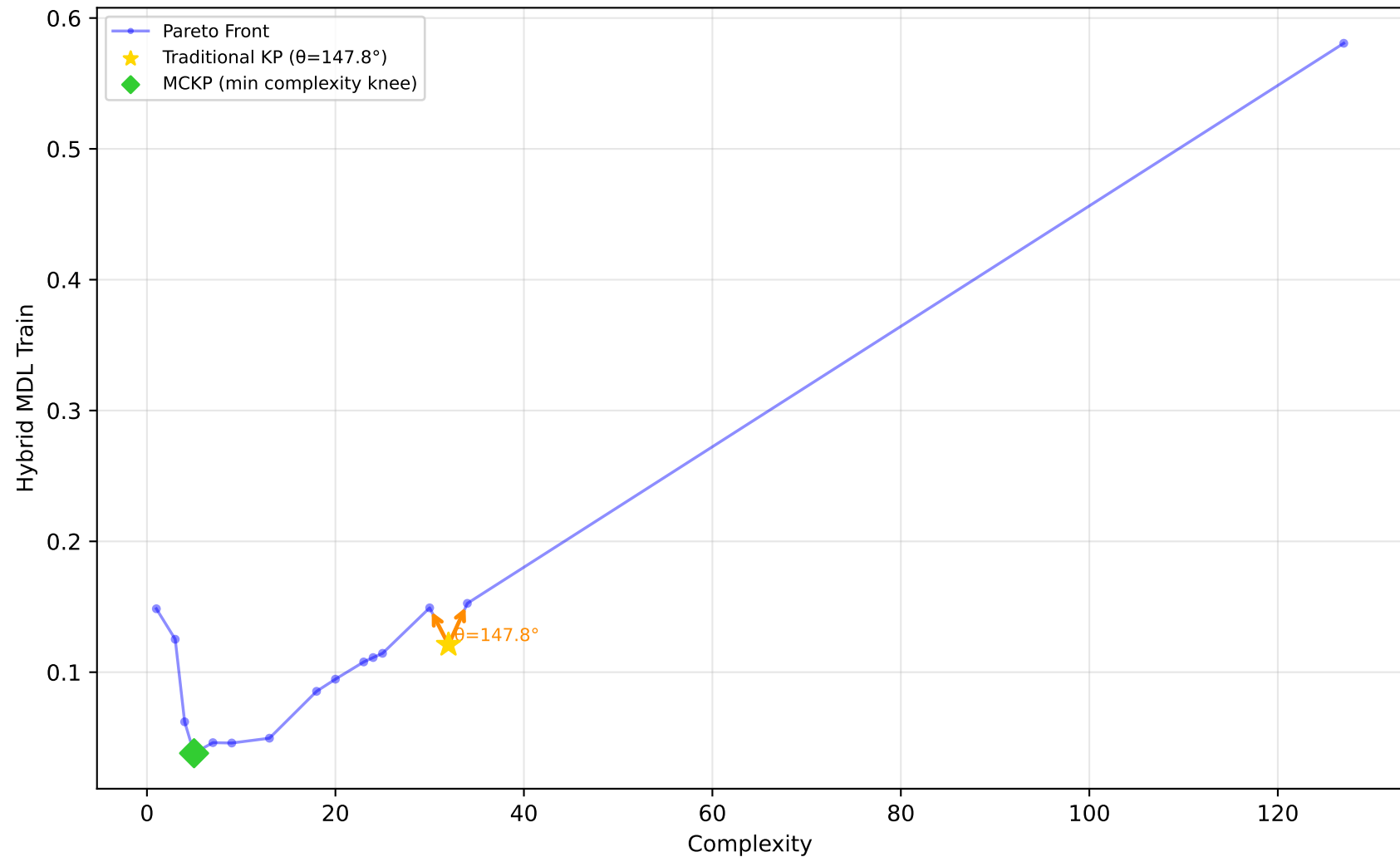
523_analcatdata_neavote - Run 24 - SVP - Hybrid MDL Train \lambda_1=0.00, \lambda_2=0.90, \lambda_3=0.00 | Difficulty: 1.00 | Method: hmr
