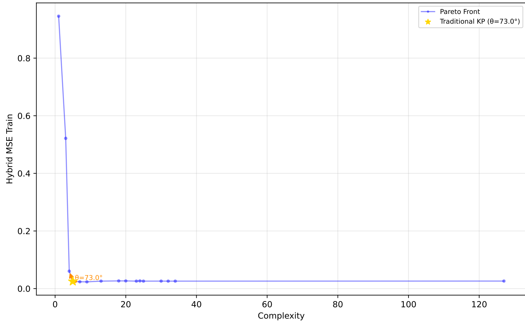
523_analcatdata_neavote - Run 24 - SVP - Hybrid MSE Train \lambda_1=0.00, \lambda_2=0.90, \lambda_3=0.00 | Difficulty: 1.00 | Method: hmr
