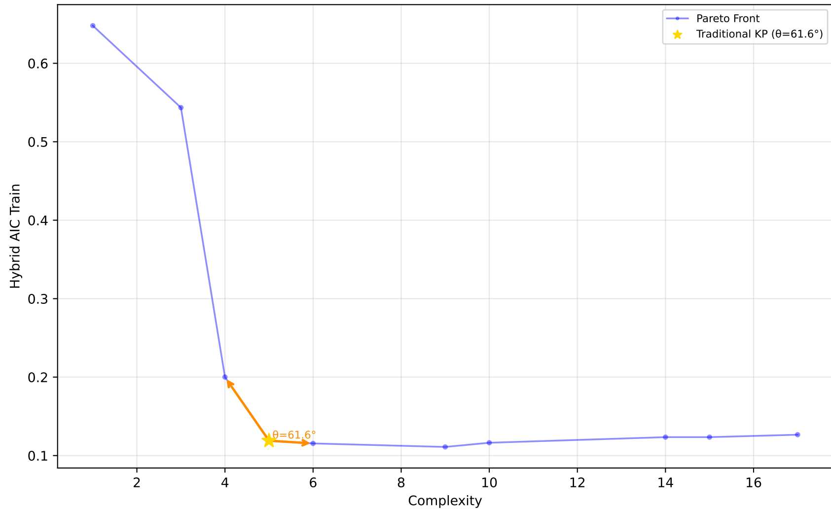
523_analcatdata_neavote - Run 25 - MVP - Hybrid AIC Train \lambda_1=0.00, \lambda_2=0.10, \lambda_3=0.00 | Difficulty: 1.00 | Method: hmr
