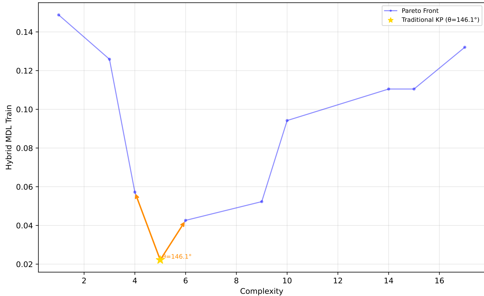
523_analcatdata_neavote - Run 25 - MVP - Hybrid MDL Train \lambda_1=0.00, \lambda_2=0.40, \lambda_3=0.00 | Difficulty: 1.00 | Method: hmr
