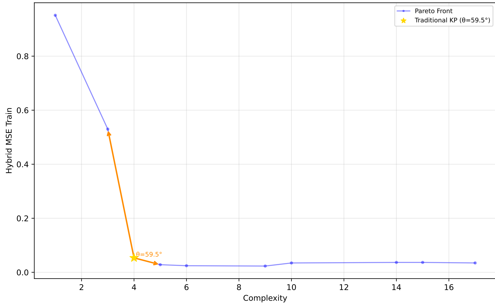
523_analcatdata_neavote - Run 25 - MVP - Hybrid MSE Train \lambda_1=0.00, \lambda_2=0.10, \lambda_3=0.00 | Difficulty: 1.00 | Method: hmr
