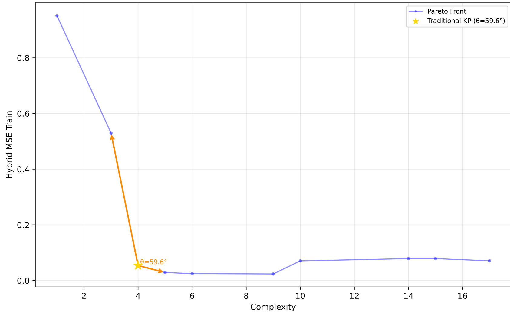
523_analcatdata_neavote - Run 25 - MVP - Hybrid MSE Train \lambda_1=0.00, \lambda_2=0.40, \lambda_3=0.00 | Difficulty: 1.00 | Method: hmr
