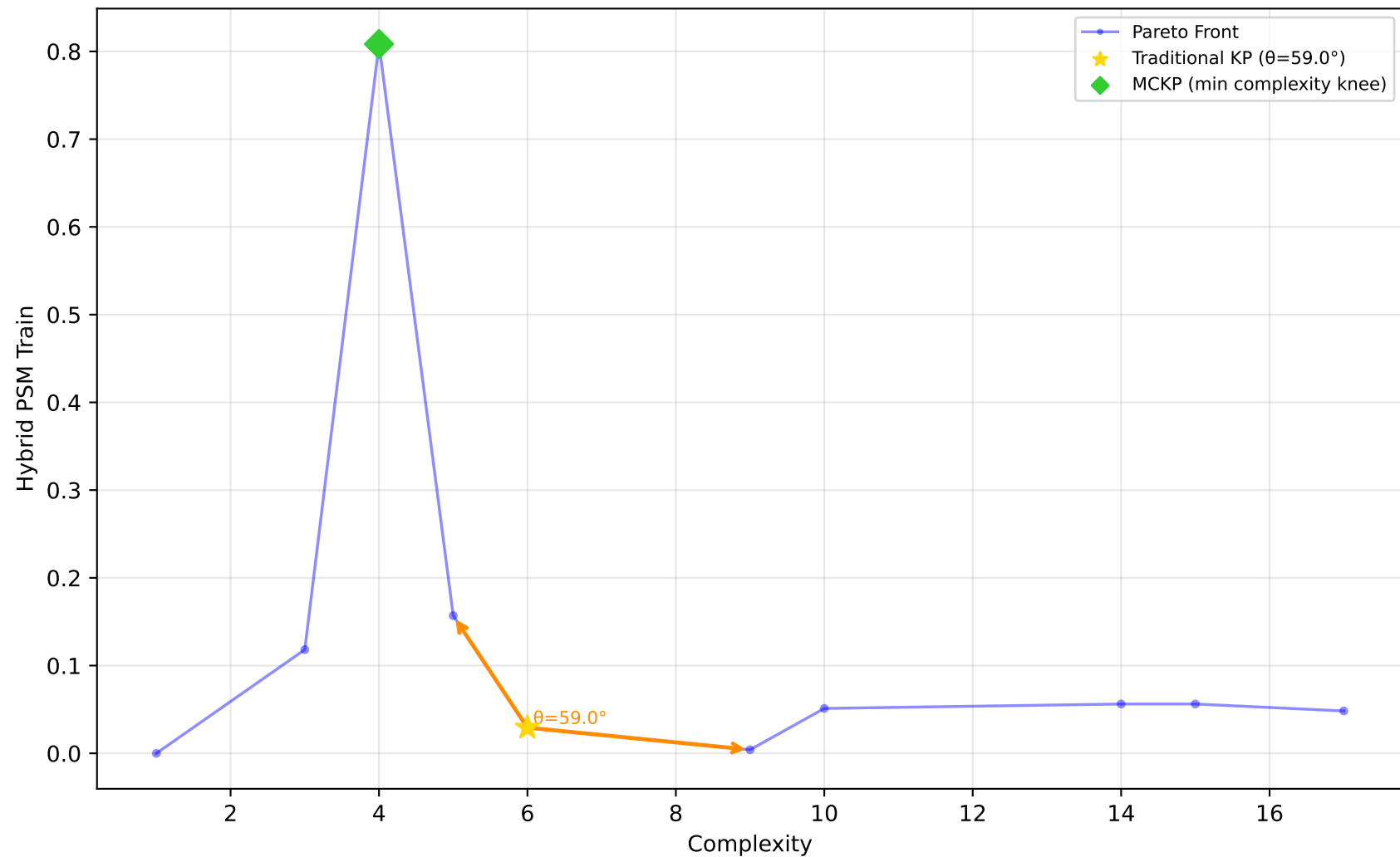
523_analcatdata_neavote - Run 25 - MVP - Hybrid PSM Train \lambda_1=0.00, \lambda_2=0.40, \lambda_3=0.00 | Difficulty: 1.00 | Method: hmr
