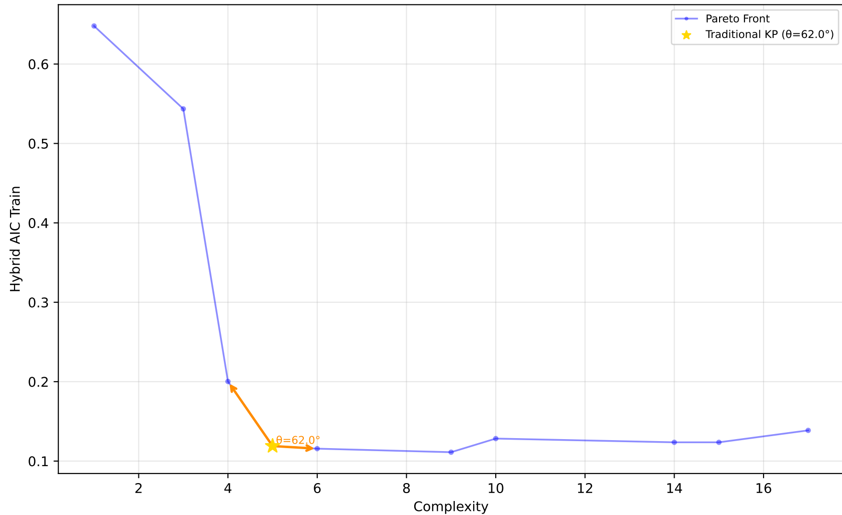
523_analcatdata_neavote - Run 25 - SVP - Hybrid AIC Train \lambda_1=0.00 , \lambda_2=0.20 , \lambda_3=0.00 | Difficulty: 1.00 | Method: hmr
