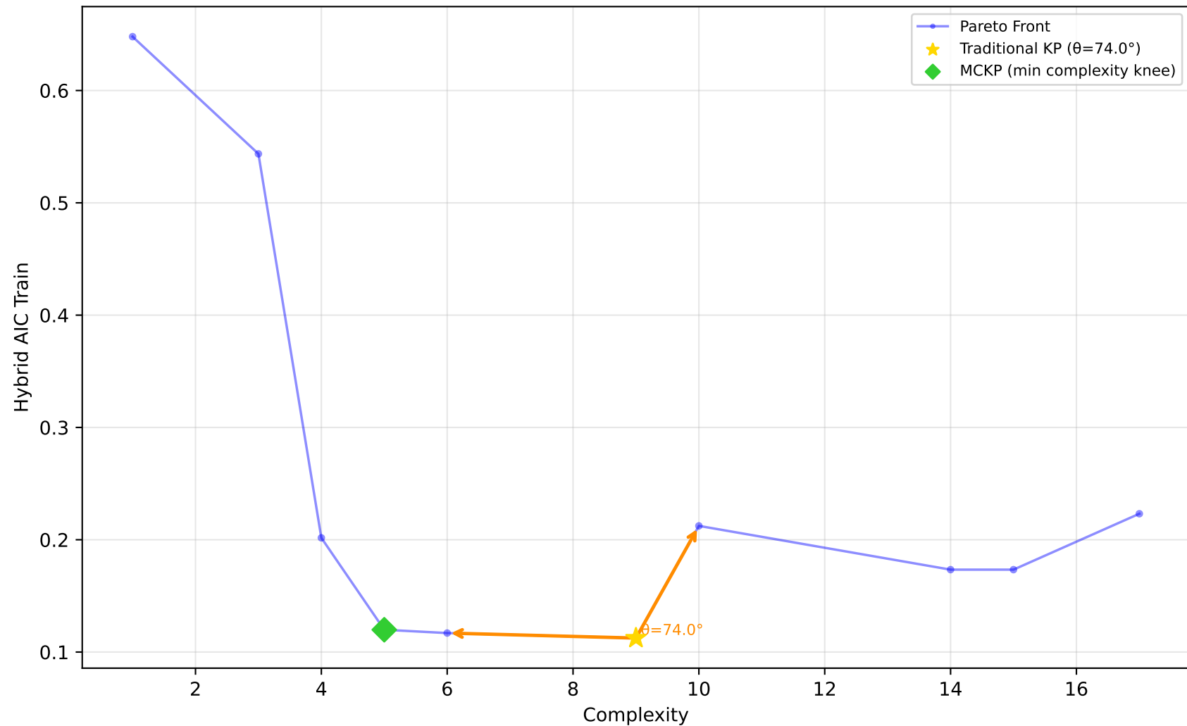
523_analcatdata_neavote - Run 25 - SVP - Hybrid AIC Train \lambda_1=0.00, \lambda_2=0.90, \lambda_3=0.00 | Difficulty: 1.00 | Method: hmr
