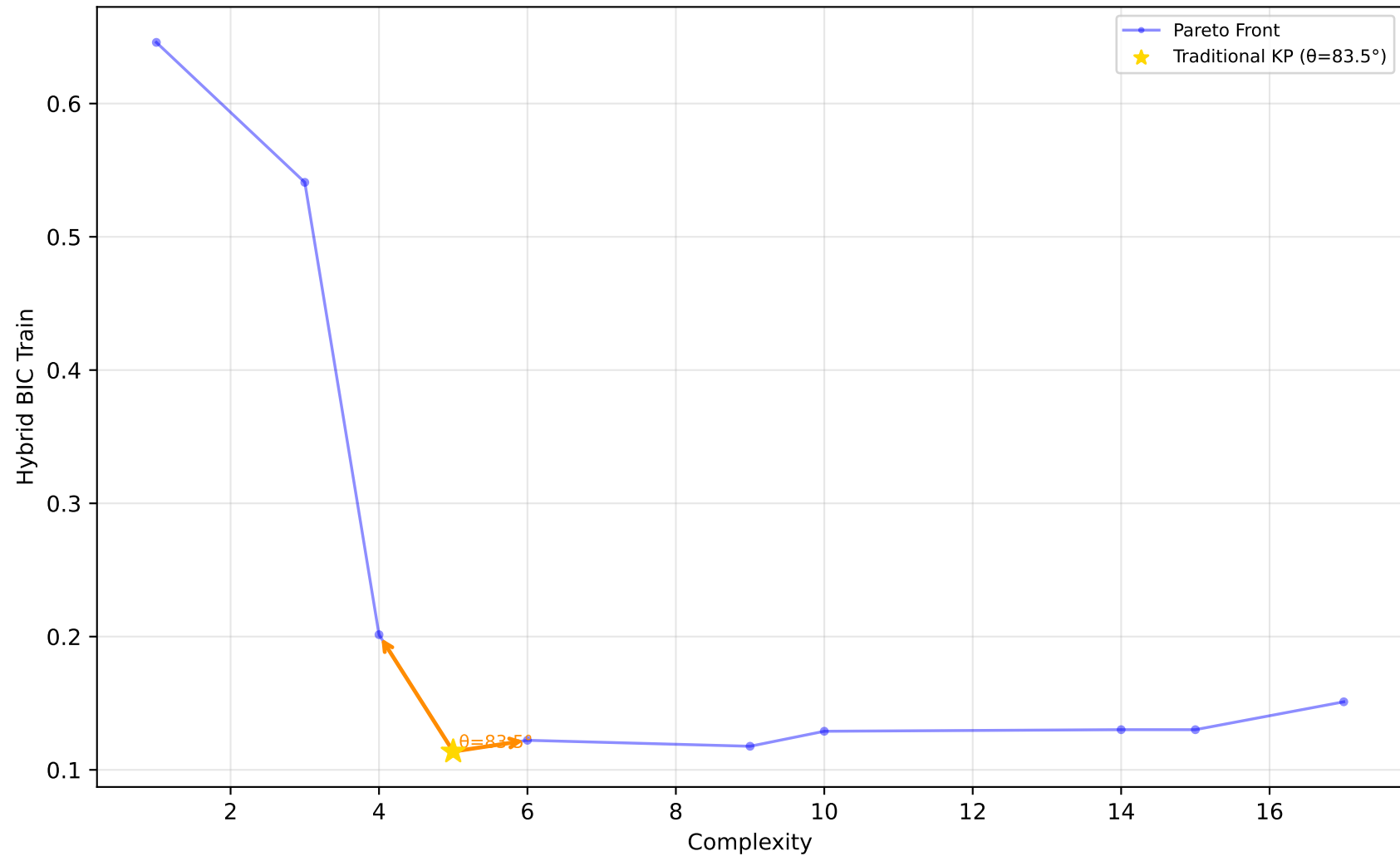
523_analcatdata_neavote - Run 25 - SVP - Hybrid BIC Train \lambda_1=0.00 , \lambda_2=0.20 , \lambda_3=0.00 | Difficulty: 1.00 | Method: hmr
