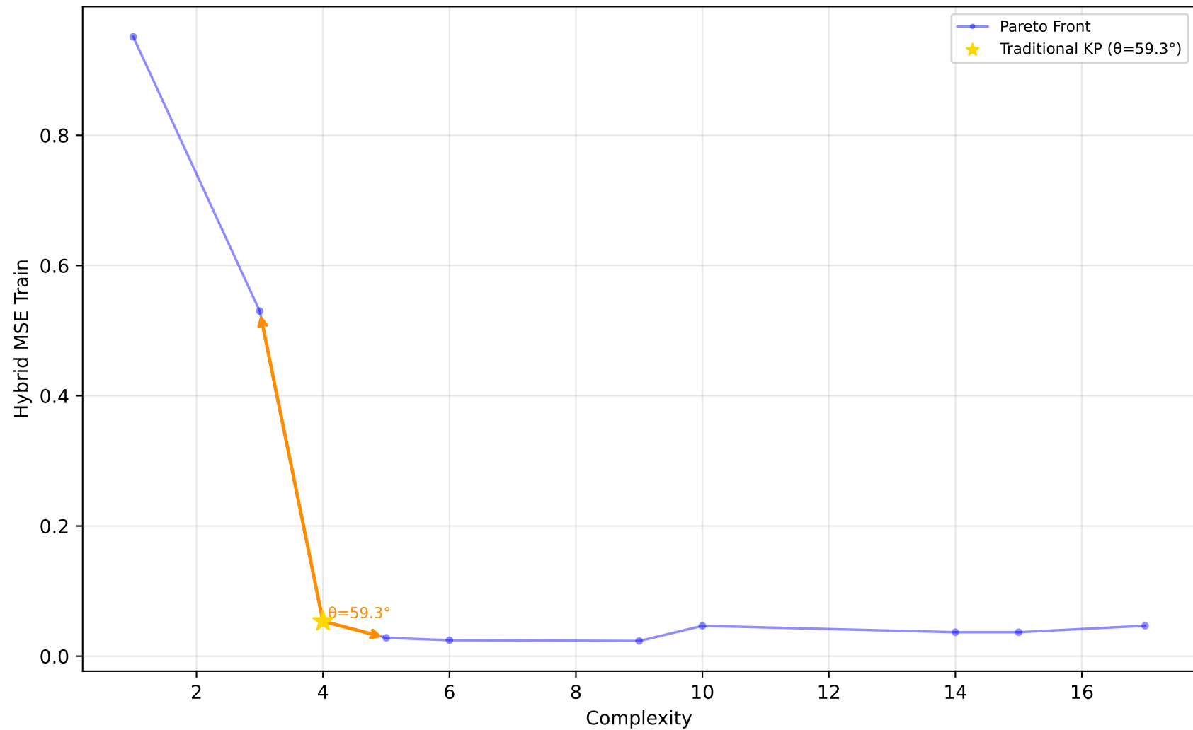
523_analcatdata_neavote - Run 25 - SVP - Hybrid MSE Train \lambda_1=0.00, \lambda_2=0.20, \lambda_3=0.00 | Difficulty: 1.00 | Method: hmr
