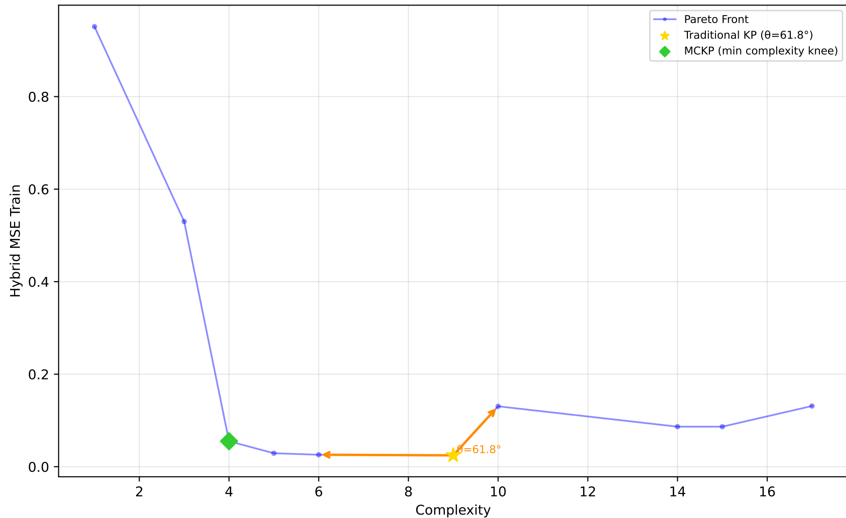
523_analcatdata_neavote - Run 25 - SVP - Hybrid MSE Train \lambda_1=0.00, \lambda_2=0.90, \lambda_3=0.00 | Difficulty: 1.00 | Method: hmr
