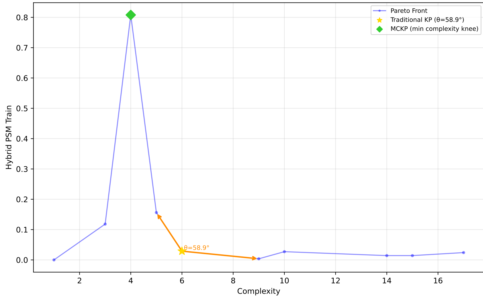
523_analcatdata_neavote - Run 25 - SVP - Hybrid PSM Train \lambda_1=0.00 , \lambda_2=0.20 , \lambda_3=0.00 | Difficulty: 1.00 | Method: hmr
