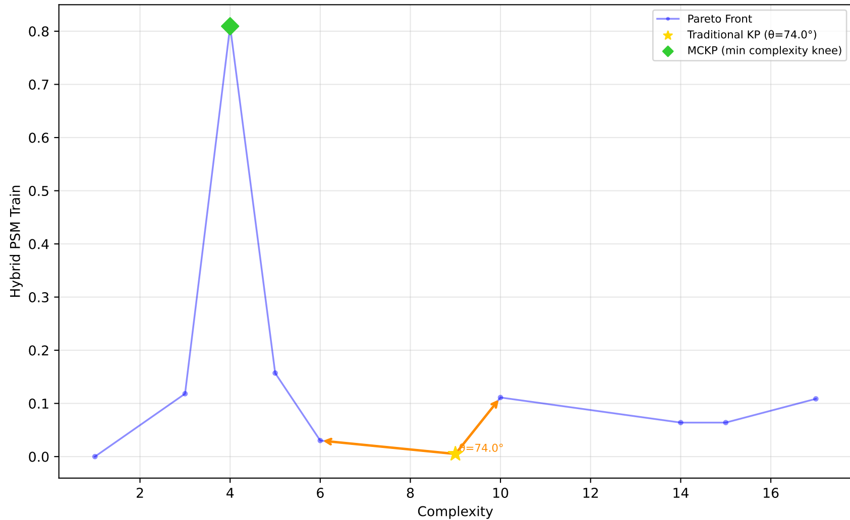
523_analcatdata_neavote - Run 25 - SVP - Hybrid PSM Train \lambda_1=0.00, \lambda_2=0.90, \lambda_3=0.00 | Difficulty: 1.00 | Method: hmr
