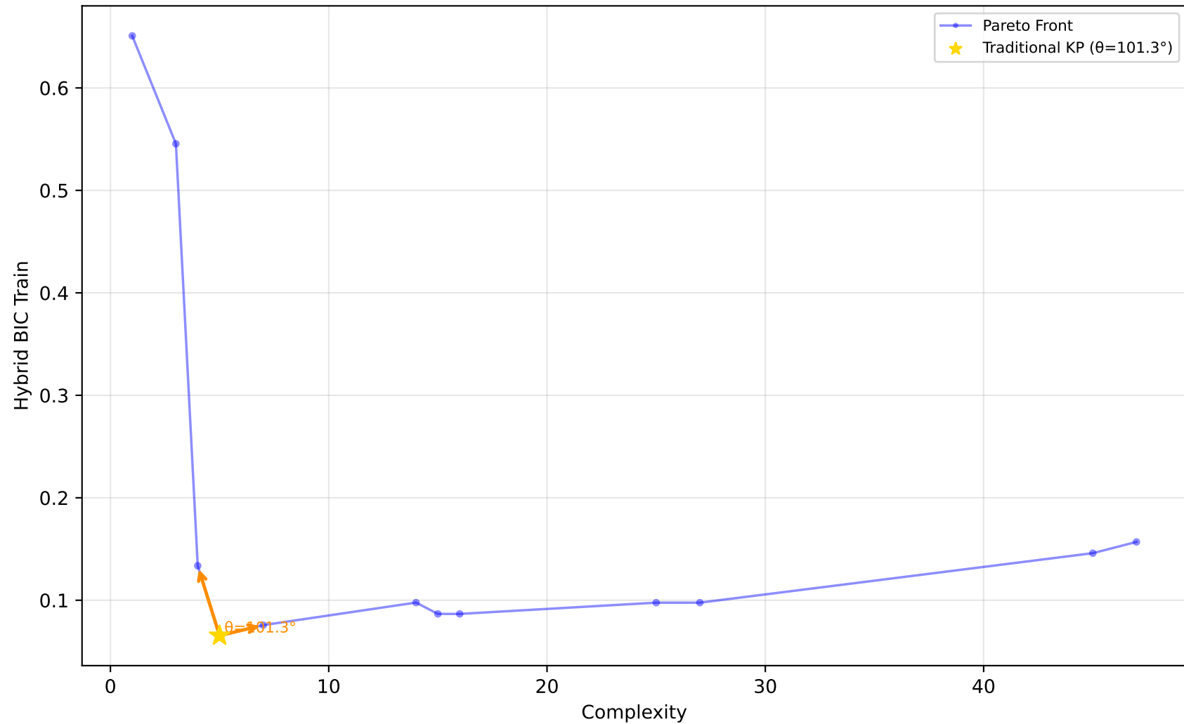
523_analcatdata_neavote - Run 26 - MVP - Hybrid BIC Train \lambda_1=0.00, \lambda_2=0.10, \lambda_3=0.00 | Difficulty: 1.00 | Method: hmr
