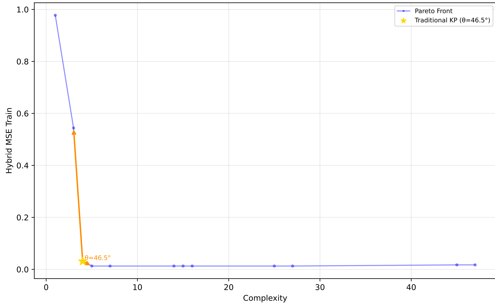
523_analcatdata_neavote - Run 26 - MVP - Hybrid MSE Train \lambda_1=0.00, \lambda_2=0.10, \lambda_3=0.00 | Difficulty: 1.00 | Method: hmr
