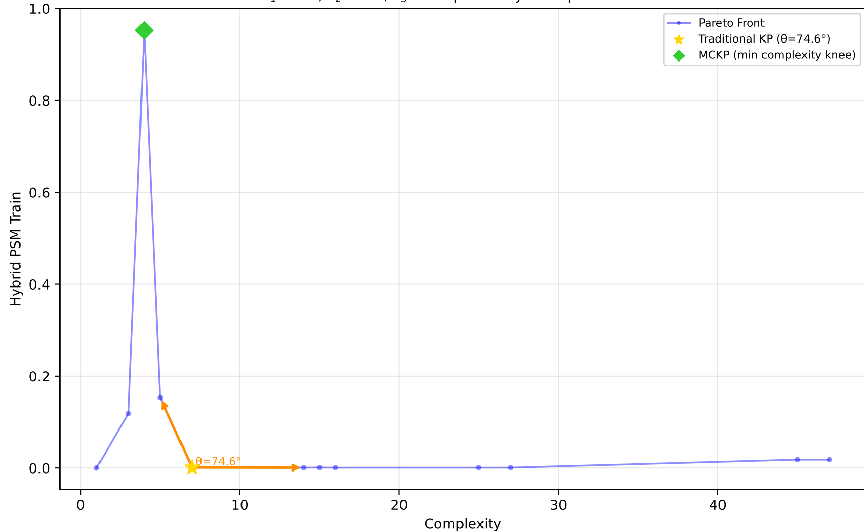
523_analcatdata_neavote - Run 26 - MVP - Hybrid PSM Train \lambda_1=0.00, \lambda_2=0.40, \lambda_3=0.00 | Difficulty: 1.00 | Method: hmr
