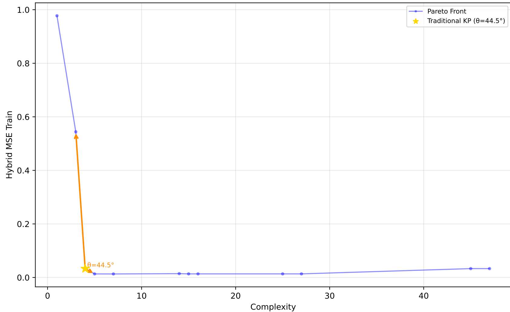
523_analcatdata_neavote - Run 26 - SVP - Hybrid MSE Train \lambda_1=0.00, \lambda_2=0.90, \lambda_3=0.00 | Difficulty: 1.00 | Method: hmr
