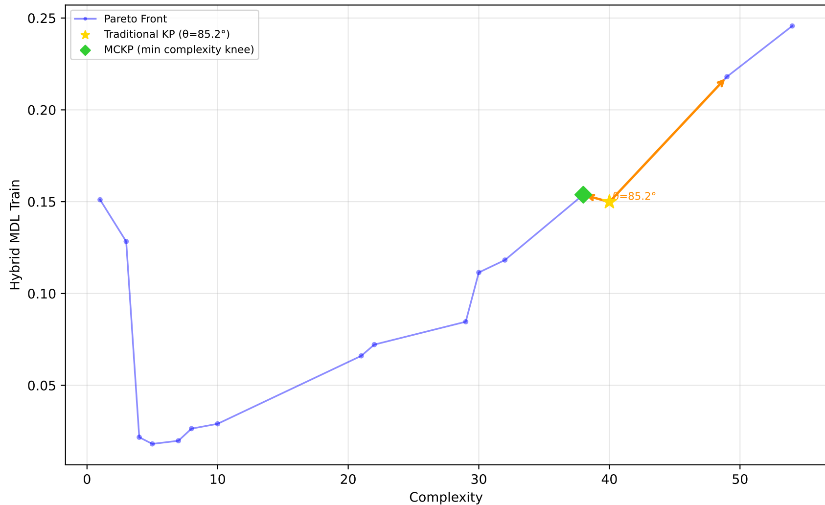
523_analcatdata_neavote - Run 27 - MVP - Hybrid MDL Train \lambda_1=0.00, \lambda_2=0.10, \lambda_3=0.00 | Difficulty: 1.00 | Method: hmr
