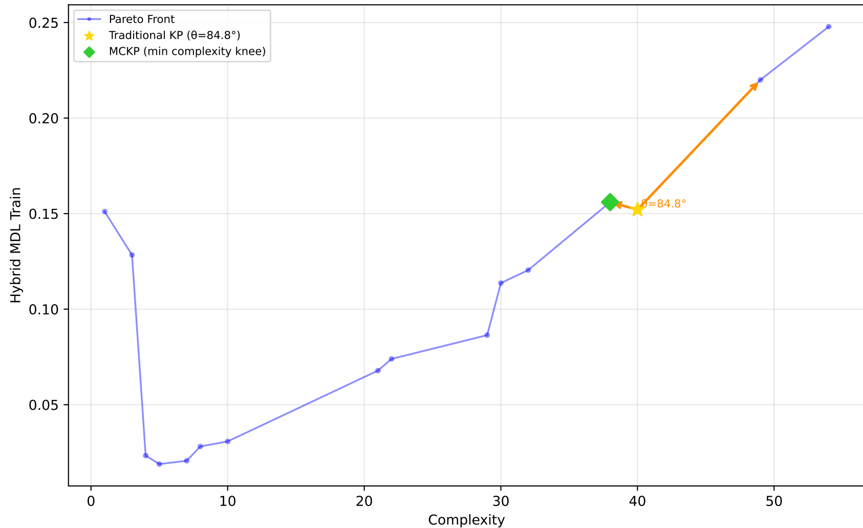
523_analcatdata_neavote - Run 27 - MVP - Hybrid MDL Train \lambda_1=0.00, \lambda_2=0.40, \lambda_3=0.00 | Difficulty: 1.00 | Method: hmr
