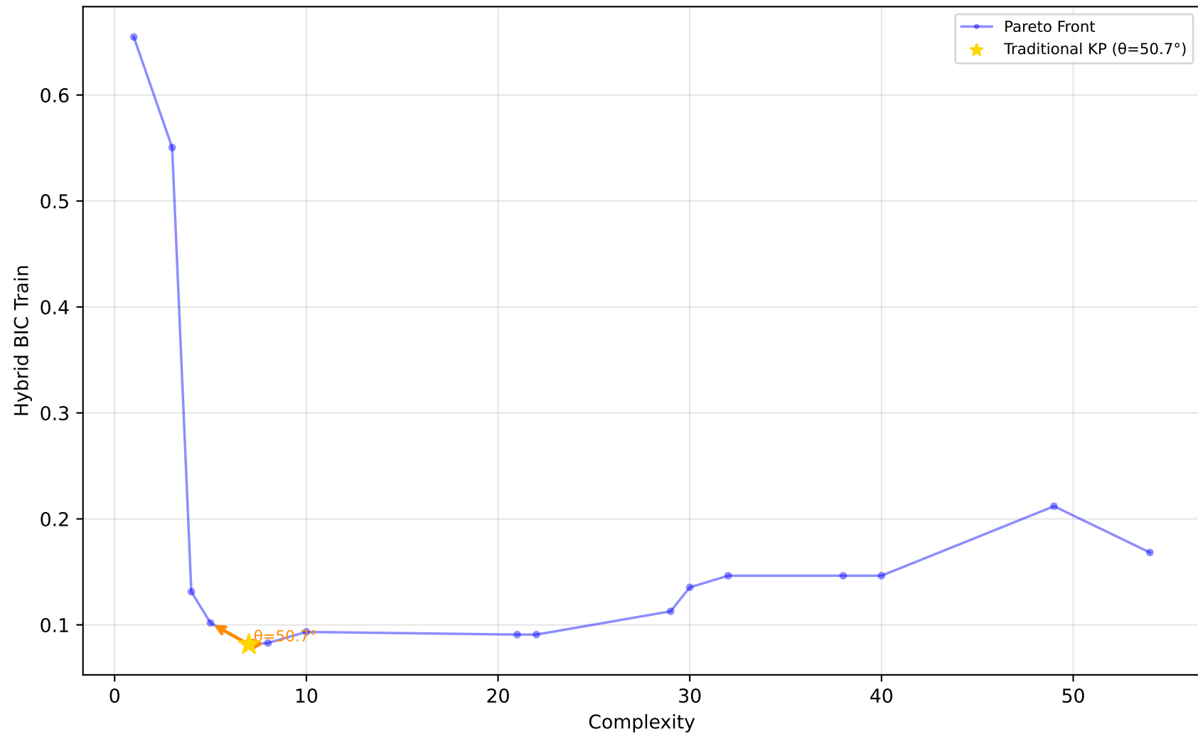
523_analcatdata_neavote - Run 27 - SVP - Hybrid BIC Train \lambda_1=0.00, \lambda_2=0.90, \lambda_3=0.00 | Difficulty: 1.00 | Method: hmr
