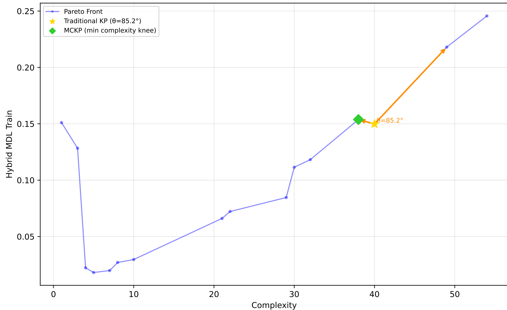
523_analcatdata_neavote - Run 27 - SVP - Hybrid MDL Train \lambda_1=0.00 , \lambda_2=0.20 , \lambda_3=0.00 | Difficulty: 1.00 | Method: hmr
