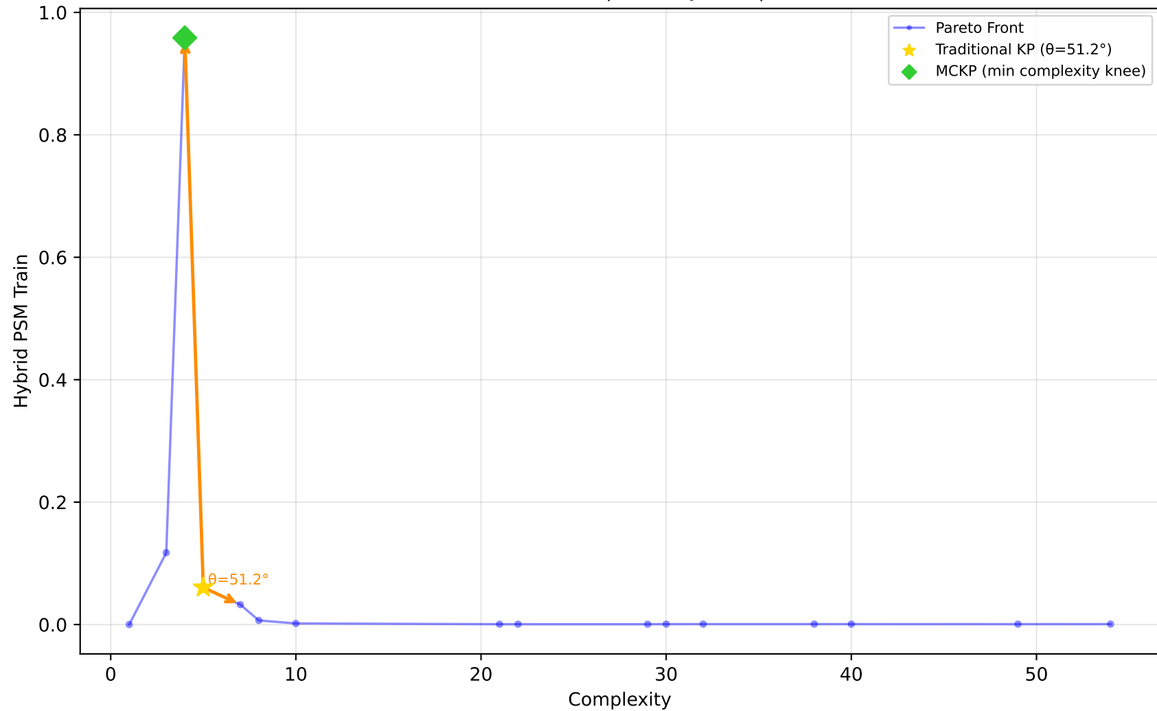
523_analcatdata_neavote - Run 27 - SVP - Hybrid PSM Train \lambda_1=0.00 , \lambda_2=0.20 , \lambda_3=0.00 | Difficulty: 1.00 | Method: hmr
