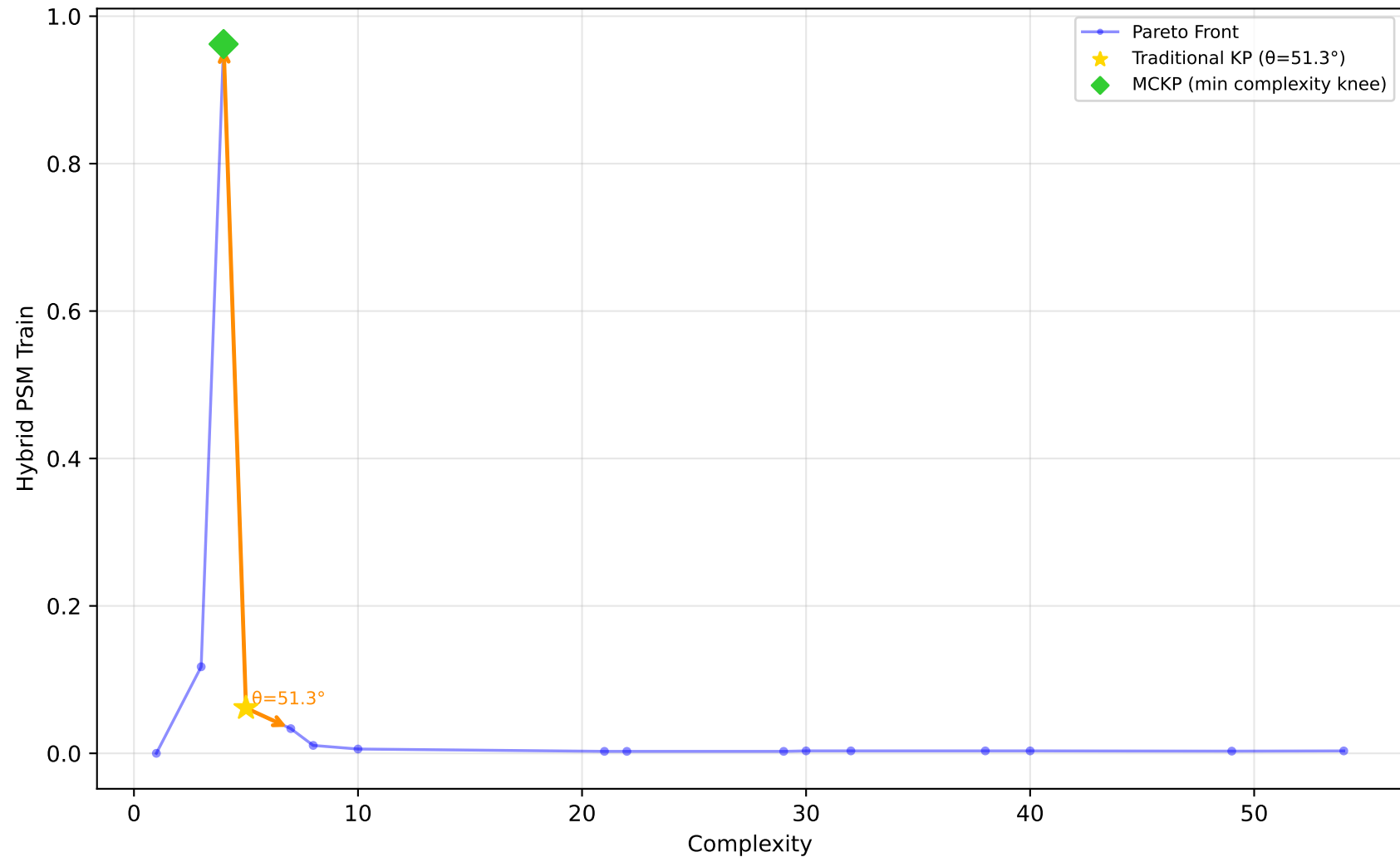
523_analcatdata_neavote - Run 27 - SVP - Hybrid PSM Train \lambda_1=0.00, \lambda_2=0.90, \lambda_3=0.00 | Difficulty: 1.00 | Method: hmr
