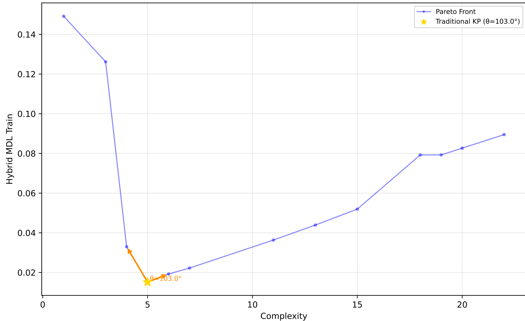
523_analcatdata_neavote - Run 28 - MVP - Hybrid MDL Train \lambda_1=0.00 , \lambda_2=0.40 , \lambda_3=0.00 | Difficulty: 1.00 | Method: hmr
