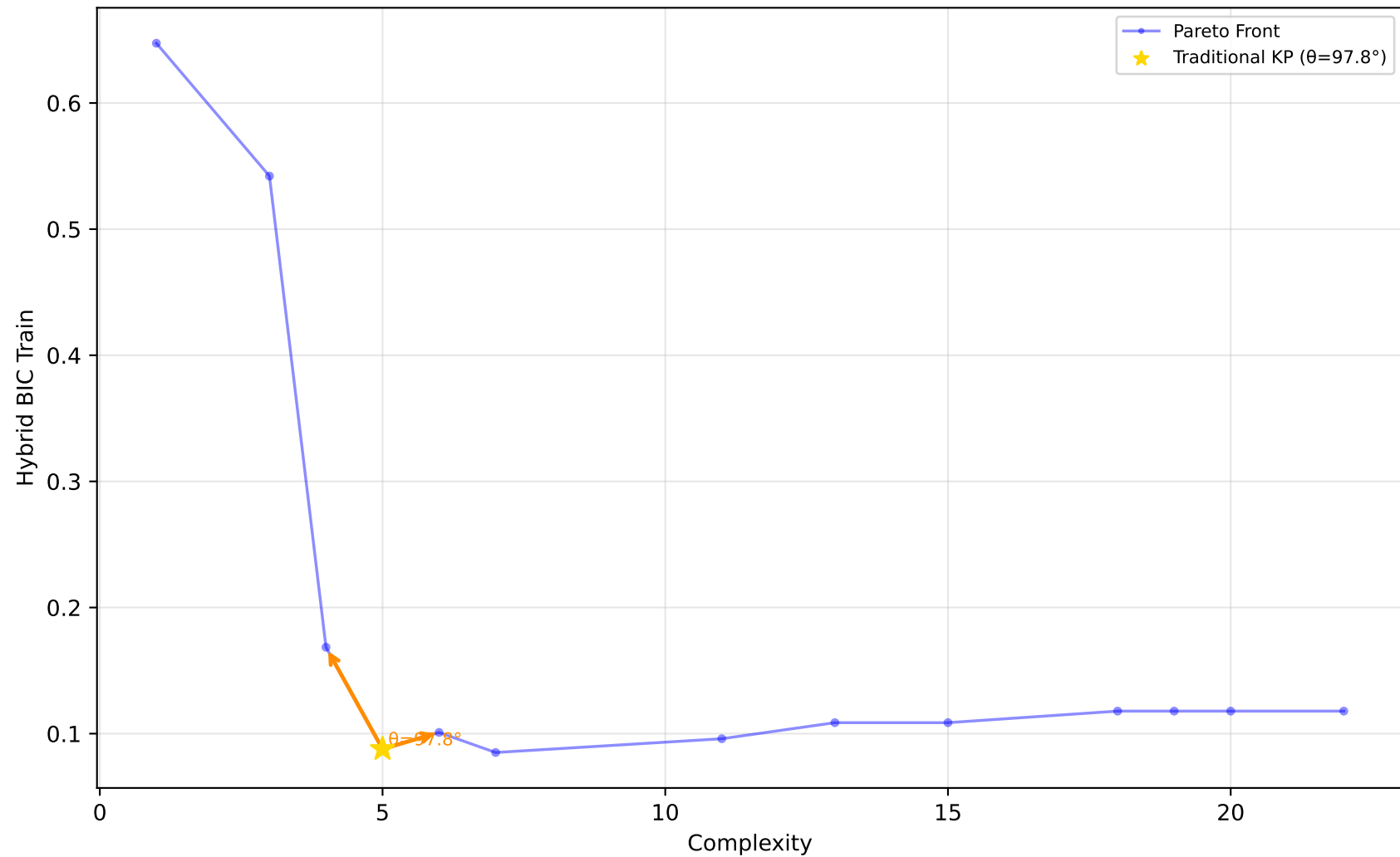
523_analcatdata_neavote - Run 28 - SVP - Hybrid BIC Train \lambda_1=0.00, \lambda_2=0.90, \lambda_3=0.00 | Difficulty: 1.00 | Method: hmr
