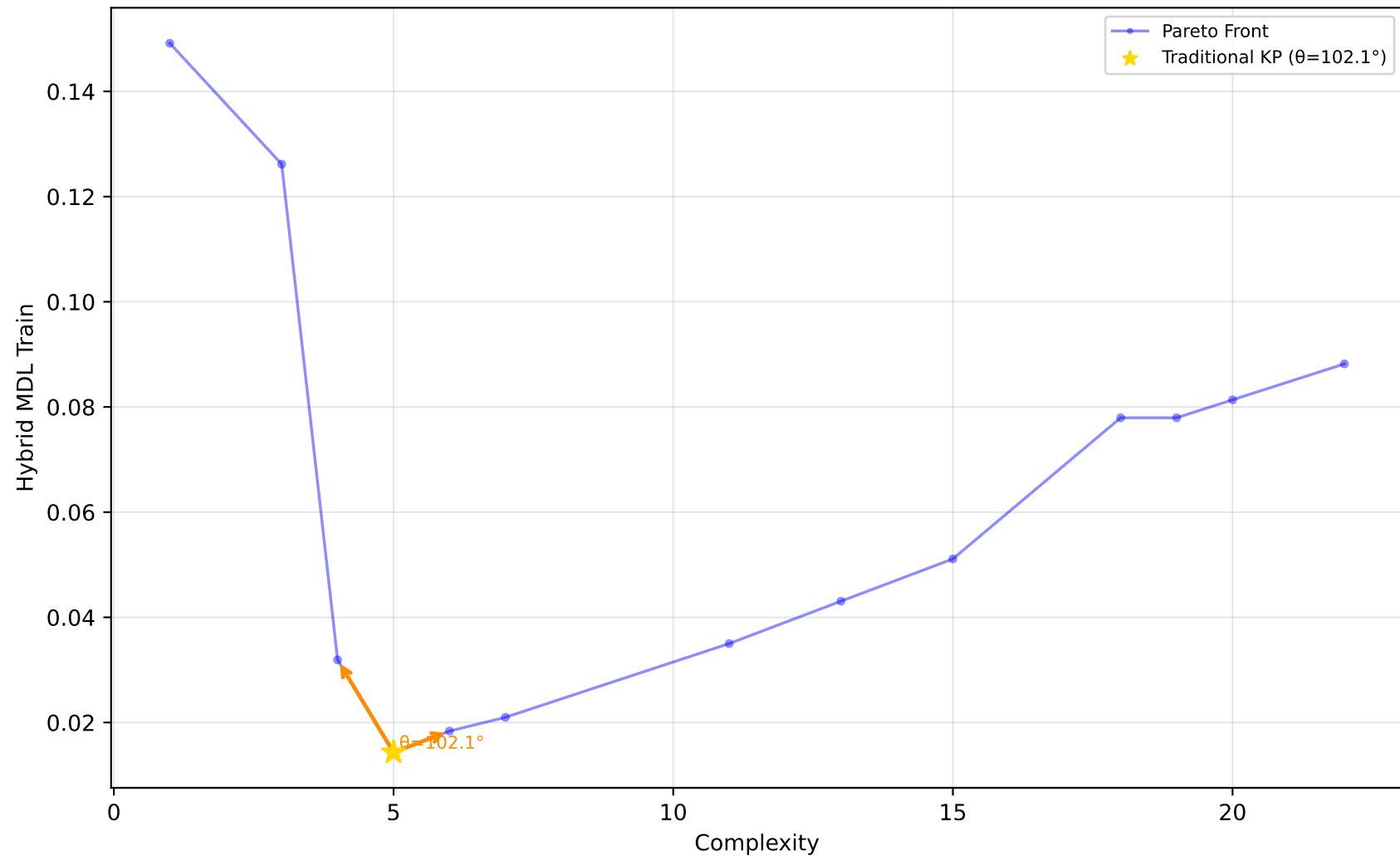
523_analcatdata_neavote - Run 28 - SVP - Hybrid MDL Train \lambda_1=0.00 , \lambda_2=0.20 , \lambda_3=0.00 | Difficulty: 1.00 | Method: hmr
