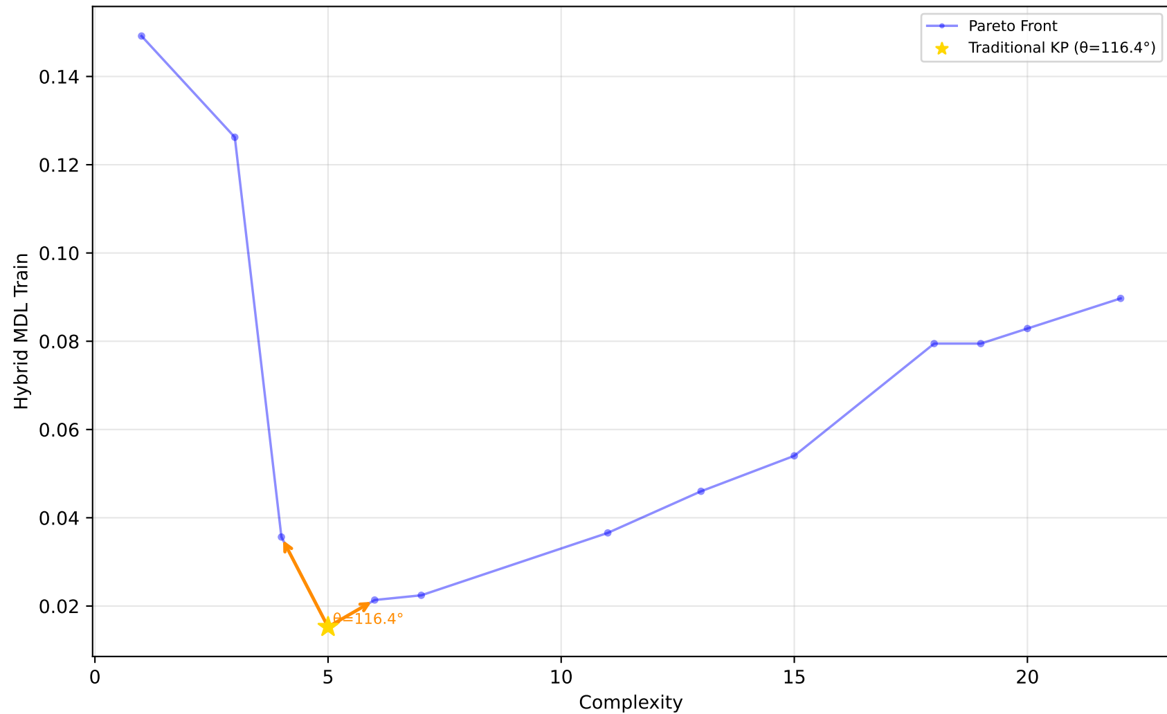
523_analcatdata_neavote - Run 28 - SVP - Hybrid MDL Train \lambda_1=0.00, \lambda_2=0.90, \lambda_3=0.00 | Difficulty: 1.00 | Method: hmr
