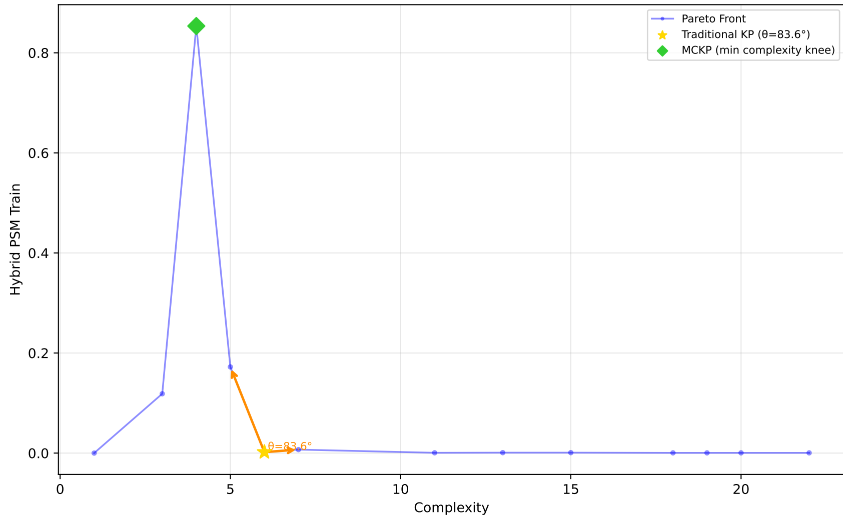
523_analcatdata_neavote - Run 28 - SVP - Hybrid PSM Train \lambda_1=0.00 , \lambda_2=0.20 , \lambda_3=0.00 | Difficulty: 1.00 | Method: hmr
