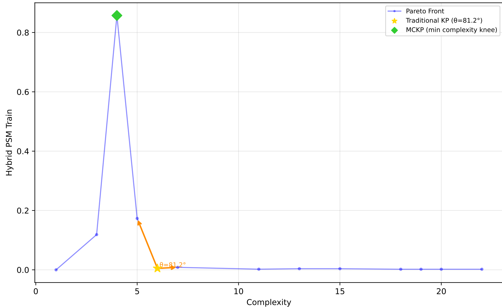
523_analcatdata_neavote - Run 28 - SVP - Hybrid PSM Train \lambda_1=0.00, \lambda_2=0.90, \lambda_3=0.00 | Difficulty: 1.00 | Method: hmr
