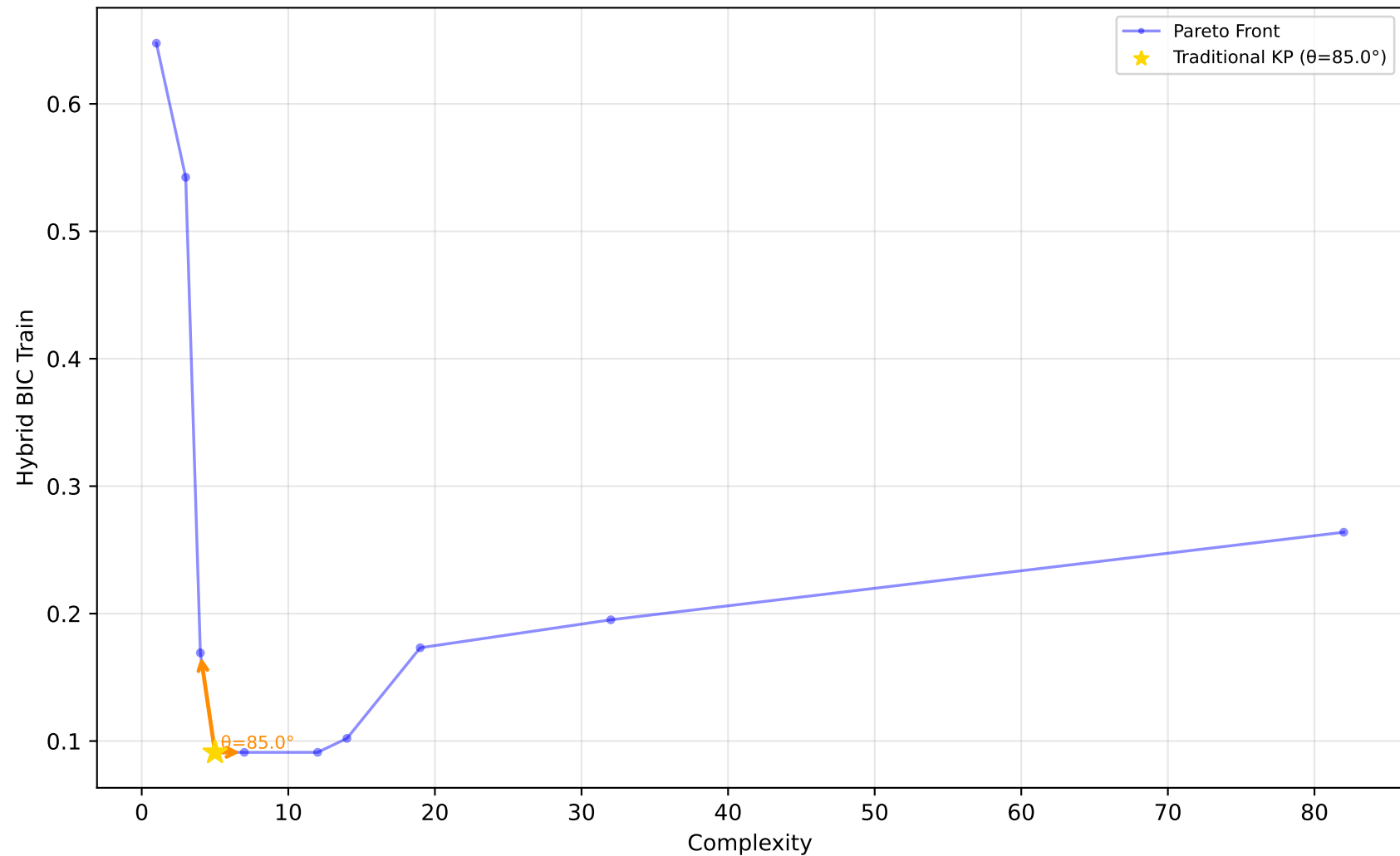
523_analcatdata_neavote - Run 29 - SVP - Hybrid BIC Train \lambda_1=0.00, \lambda_2=0.20, \lambda_3=0.00 | Difficulty: 1.00 | Method: hmr
