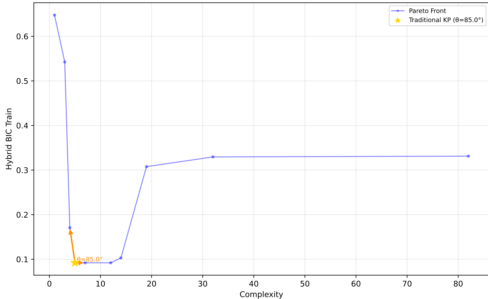
523_analcatdata_neavote - Run 29 - SVP - Hybrid BIC Train \lambda_1=0.00, \lambda_2=0.90, \lambda_3=0.00 | Difficulty: 1.00 | Method: hmr
