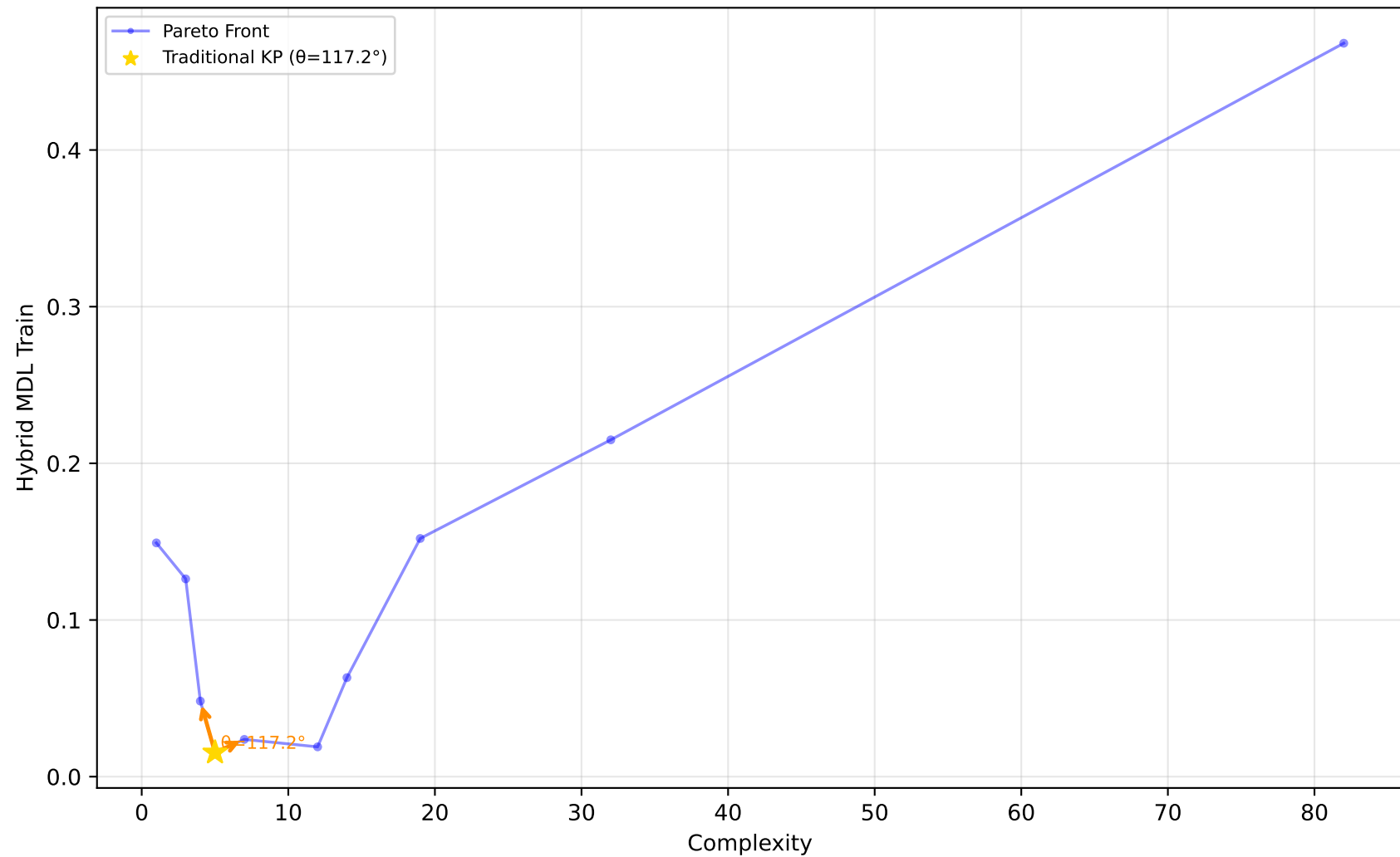
523_analcatdata_neavote - Run 29 - SVP - Hybrid MDL Train \lambda_1=0.00, \lambda_2=0.20, \lambda_3=0.00 | Difficulty: 1.00 | Method: hmr
