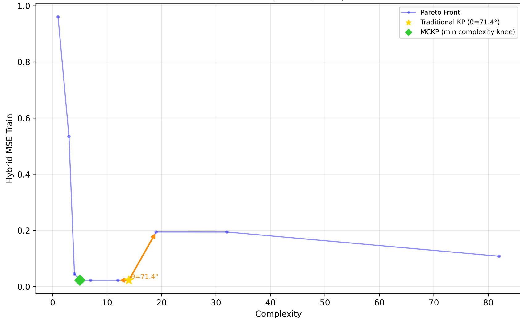
523_analcatdata_neavote - Run 29 - SVP - Hybrid MSE Train \lambda_1=0.00, \lambda_2=0.90, \lambda_3=0.00 | Difficulty: 1.00 | Method: hmr
