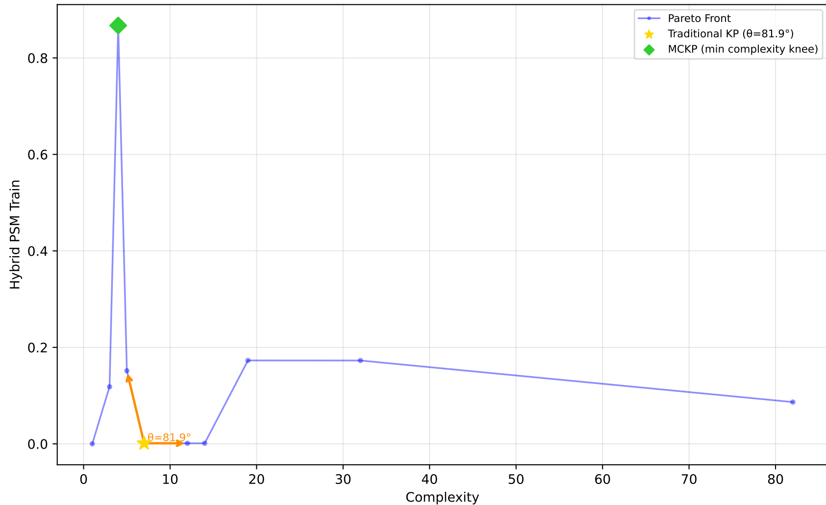
523_analcatdata_neavote - Run 29 - SVP - Hybrid PSM Train \lambda_1=0.00, \lambda_2=0.90, \lambda_3=0.00 | Difficulty: 1.00 | Method: hmr
