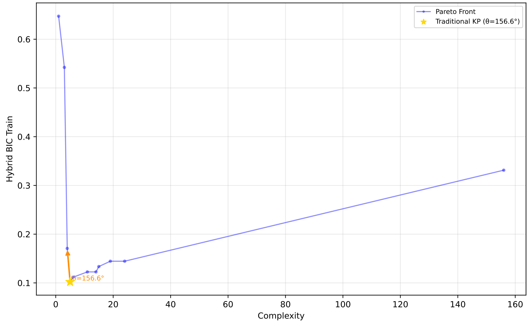
523_analcatdata_neavote - Run 2 - MVP - Hybrid BIC Train \lambda_1=0.00, \lambda_2=0.10, \lambda_3=0.00 | Difficulty: 1.00 | Method: hmr
