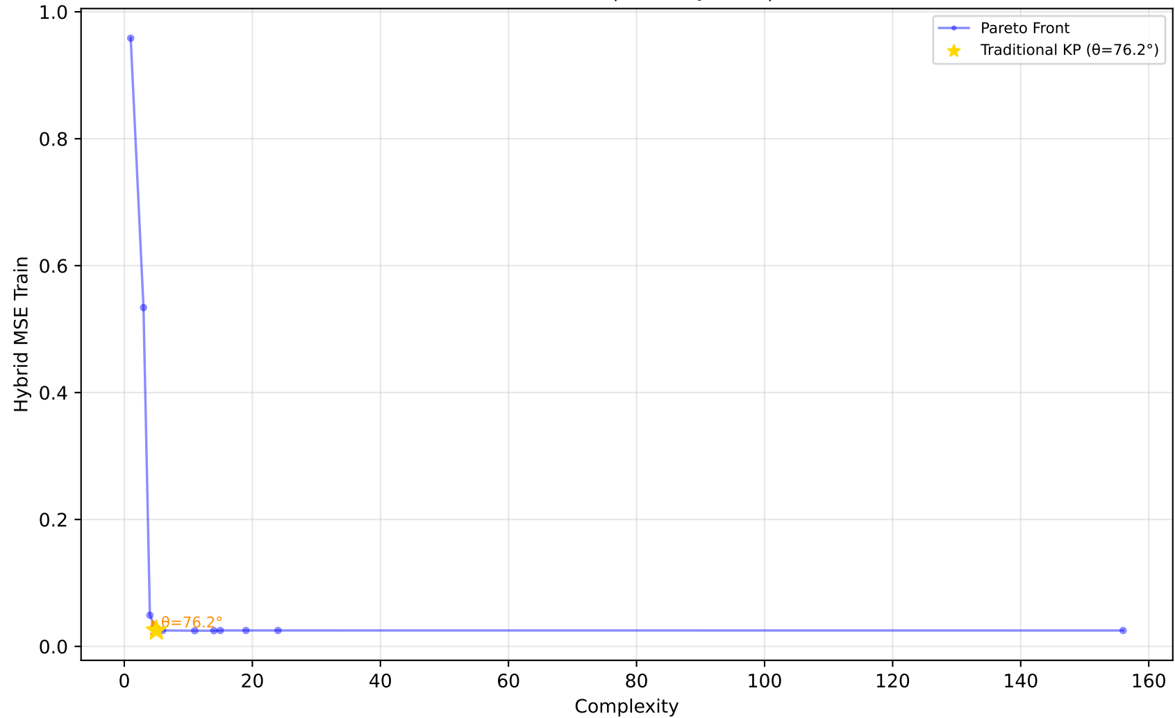
523_analcatdata_neavote - Run 2 - SVP - Hybrid MSE Train \lambda_1=0.00 , \lambda_2=0.20 , \lambda_3=0.00 | Difficulty: 1.00 | Method: hmr
