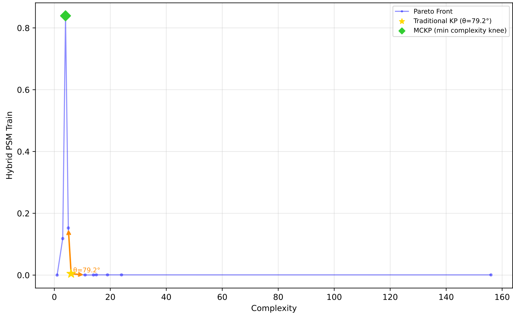
523_analcatdata_neavote - Run 2 - SVP - Hybrid PSM Train \lambda_1=0.00, \lambda_2=0.20, \lambda_3=0.00 | Difficulty: 1.00 | Method: hmr
