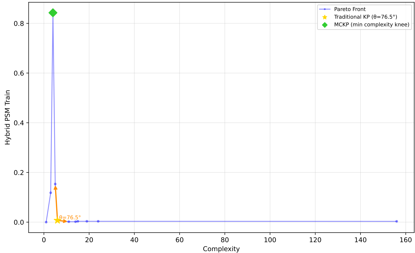
523_analcatdata_neavote - Run 2 - SVP - Hybrid PSM Train \lambda_1=0.00, \lambda_2=0.90, \lambda_3=0.00 | Difficulty: 1.00 | Method: hmr
