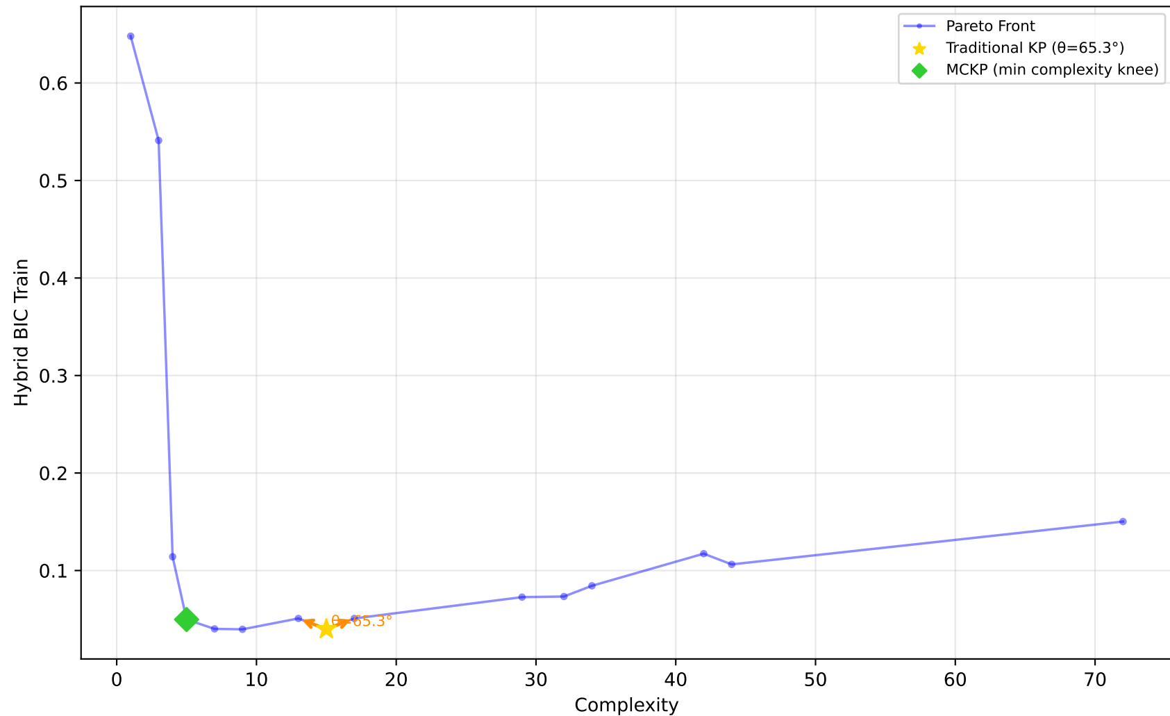
523_analcatdata_neavote - Run 30 - MVP - Hybrid BIC Train \lambda_1=0.00, \lambda_2=0.10, \lambda_3=0.00 | Difficulty: 1.00 | Method: hmr
