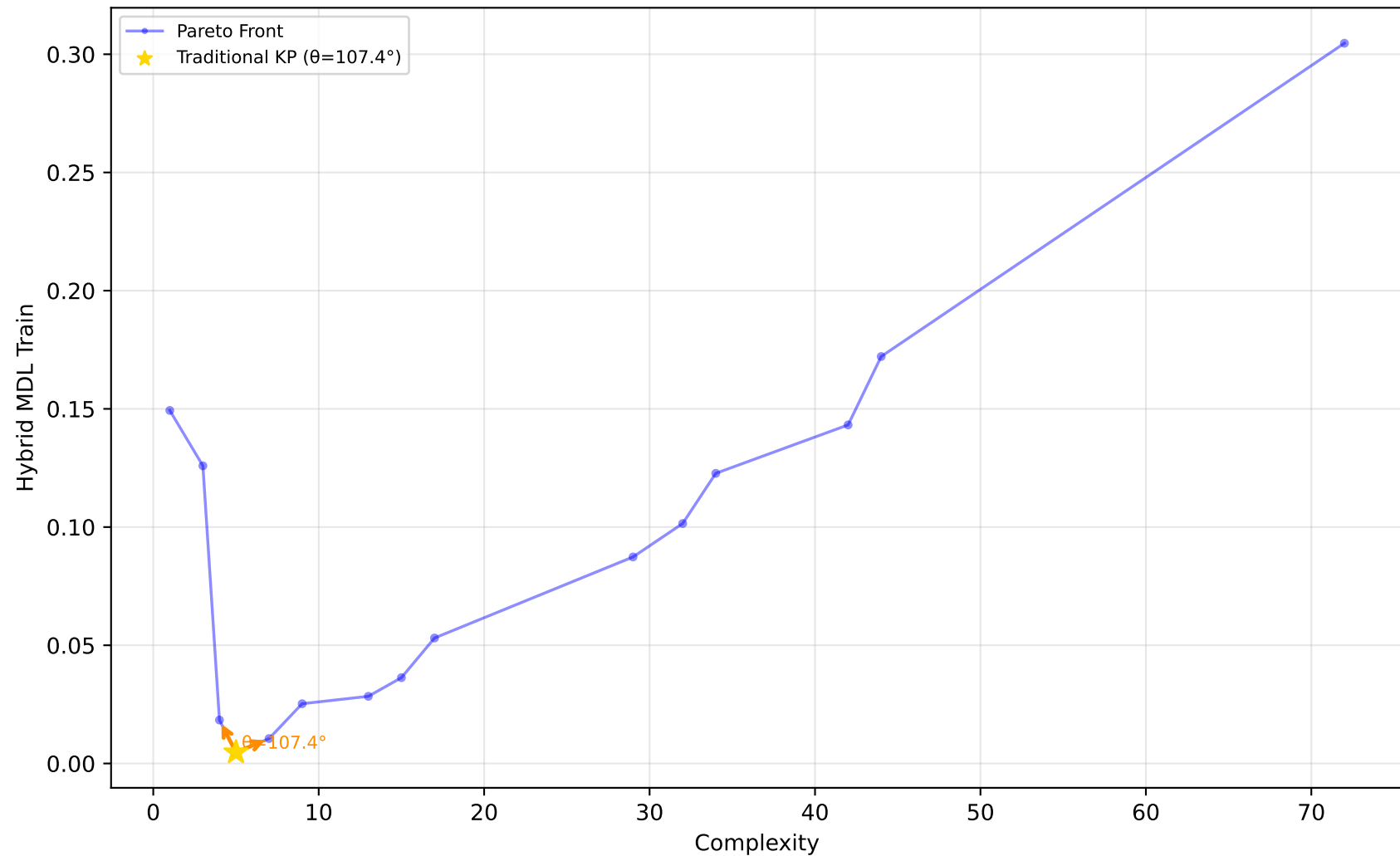
523_analcatdata_neavote - Run 30 - MVP - Hybrid MDL Train \lambda_1=0.00, \lambda_2=0.10, \lambda_3=0.00 | Difficulty: 1.00 | Method: hmr
