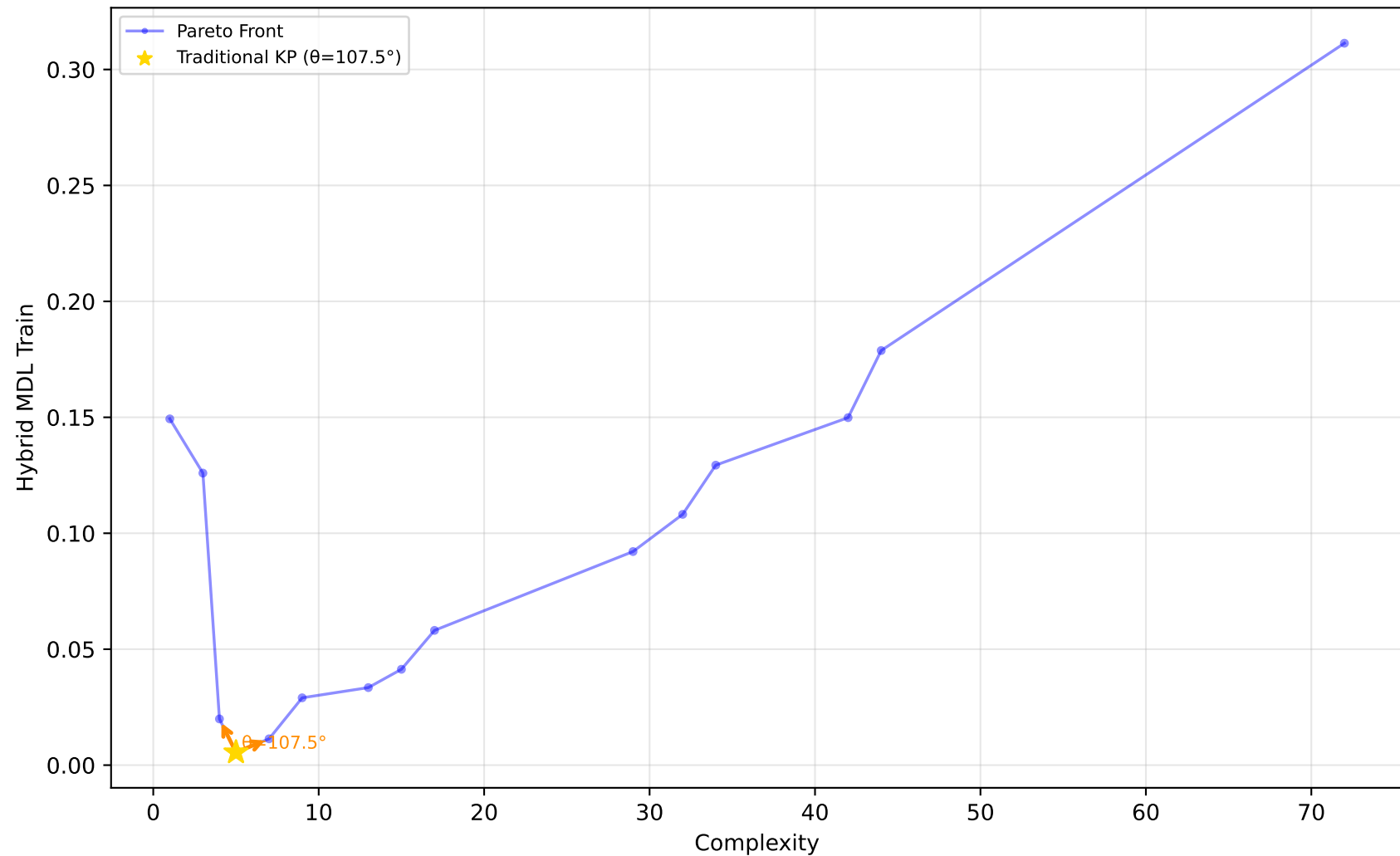
523_analcatdata_neavote - Run 30 - MVP - Hybrid MDL Train \lambda_1=0.00, \lambda_2=0.40, \lambda_3=0.00 | Difficulty: 1.00 | Method: hmr
