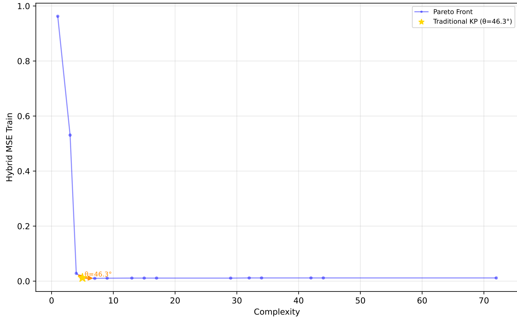
523_analcatdata_neavote - Run 30 - MVP - Hybrid MSE Train \lambda_1=0.00, \lambda_2=0.10, \lambda_3=0.00 | Difficulty: 1.00 | Method: hmr
