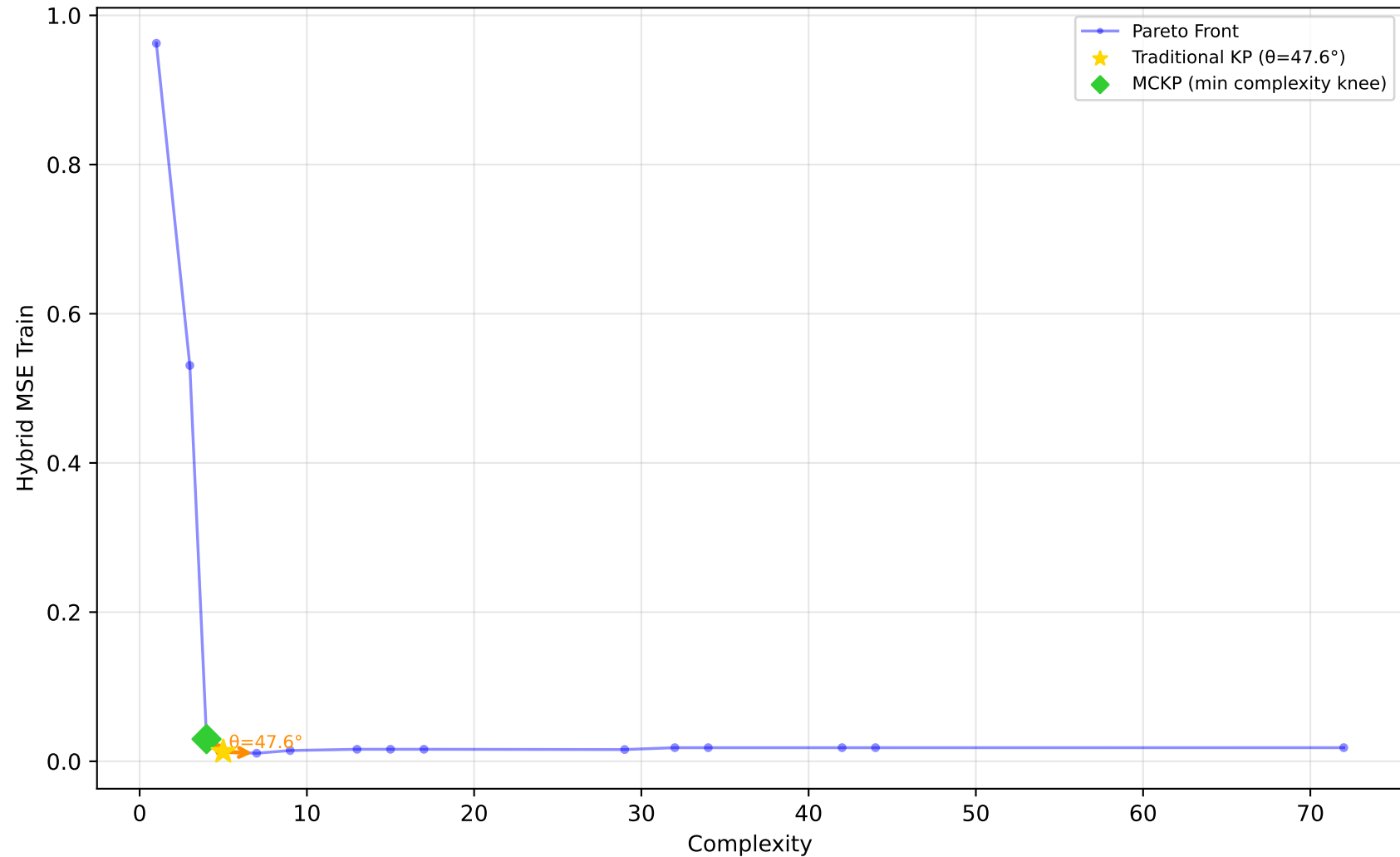
523_analcatdata_neavote - Run 30 - MVP - Hybrid MSE Train \lambda_1=0.00, \lambda_2=0.40, \lambda_3=0.00 | Difficulty: 1.00 | Method: hmr
