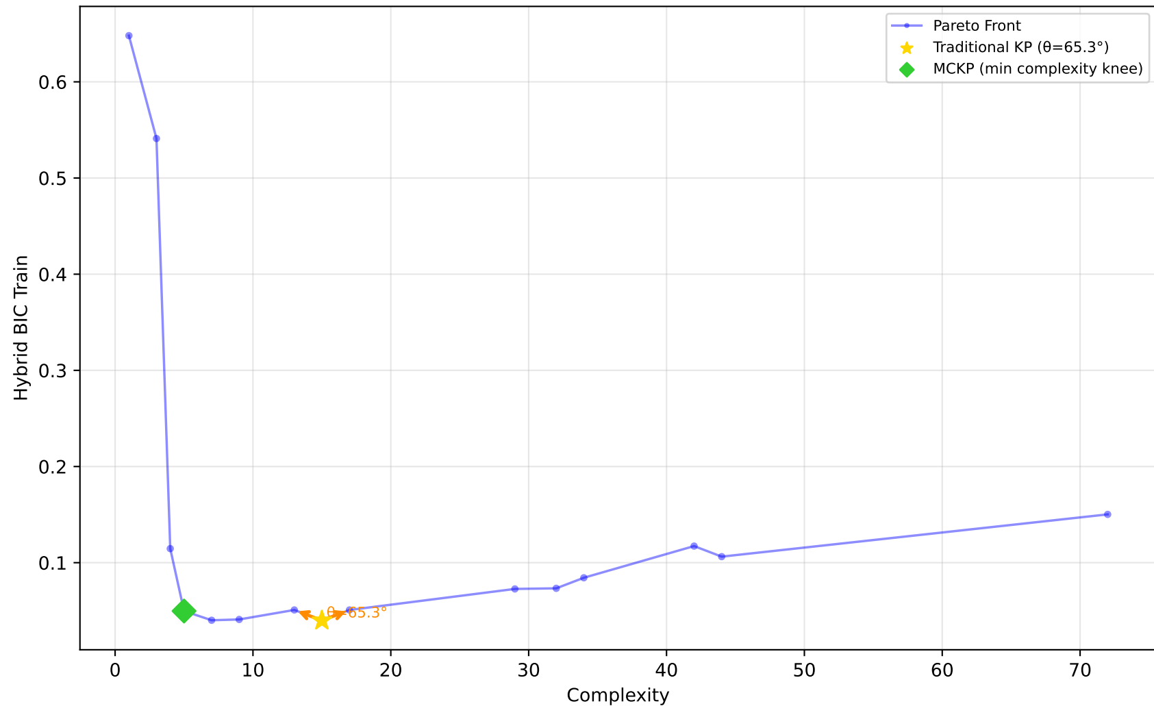
523_analcatdata_neavote - Run 30 - SVP - Hybrid BIC Train \lambda_1=0.00, \lambda_2=0.20, \lambda_3=0.00 | Difficulty: 1.00 | Method: hmr
