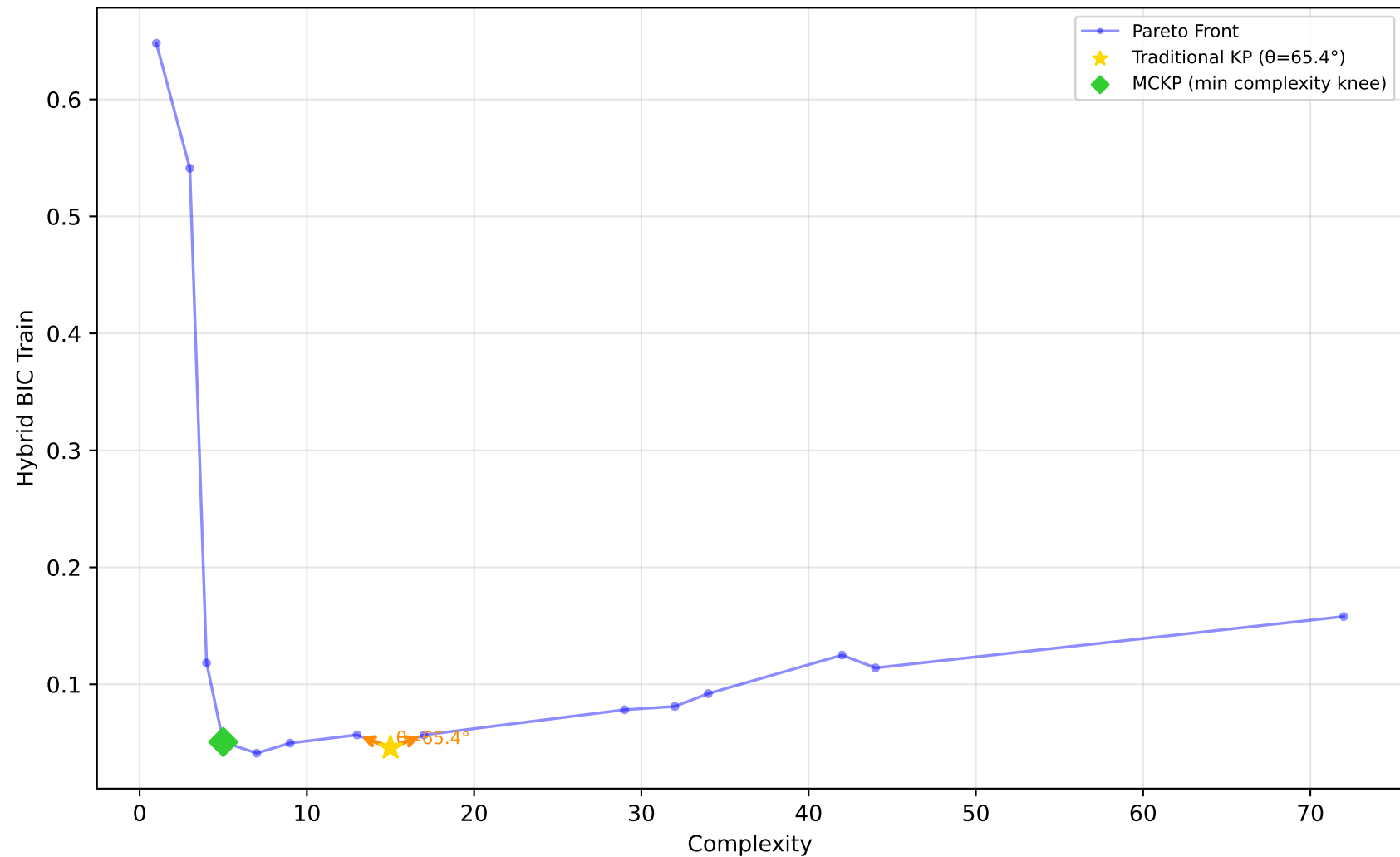
523_analcatdata_neavote - Run 30 - SVP - Hybrid BIC Train \lambda_1=0.00, \lambda_2=0.90, \lambda_3=0.00 | Difficulty: 1.00 | Method: hmr
