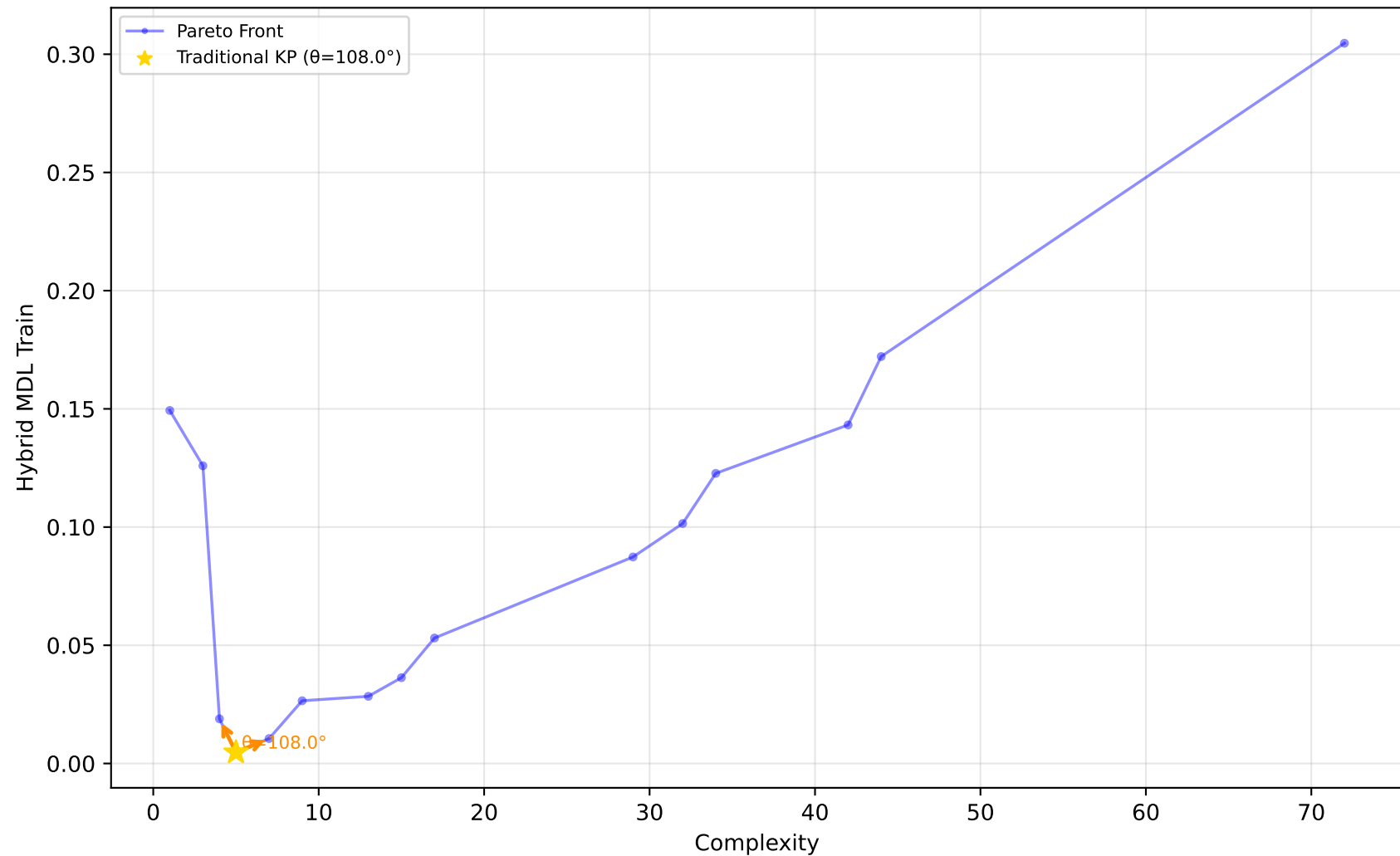
523_analcatdata_neavote - Run 30 - SVP - Hybrid MDL Train \lambda_1=0.00 , \lambda_2=0.20 , \lambda_3=0.00 | Difficulty: 1.00 | Method: hmr
